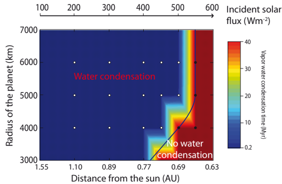
Fig. 1. Diagram showing condition for condensation of water vapor as a function of radius of the planet and solar flux. Color scale shows times at which condensation occurs. Time increases from blue to red.
