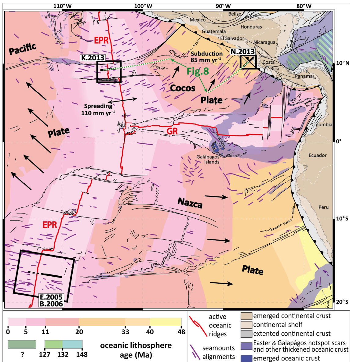
Figure 2. Synthetic map of the Eastern Pacific Ocean. Simplified map built from [19,20] and Google Earth. The spreading rate at the EPR is estimated to 11 \text{cm}\cdot\text{yr}^{-1} for the Cocos Plate [21] and 10–15 \text{cm}\cdot\text{yr}^{-1} for the Nazca Plate [22]. Large black arrows indicate plate motion direction. MT surveys: EPR = East Pacific Rise; GR = Galápagos Ridge. References: B.2006 = [2]; E.2005 = [1]; K.2013 = [21]; N.2013 = [3].
