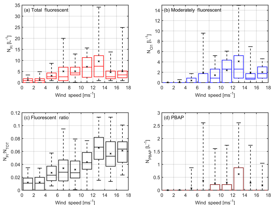
Figure 5. Fluorescent particle concentrations as a function of wind speed for the period 22–25 November 2015 for (a) total fluorescent particles, N_{FL} ; (b) moderately fluorescent particles, N_{C11} ; (c) ratio of total fluorescent particles to total particle concentration N_{FL} : N_{TOT} ; and (d) N_{PBAP} ( N_{C12} + N_{C14} ).
