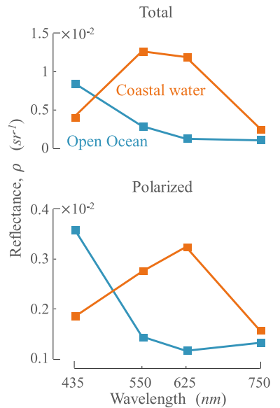
Fig. 13. The estimated total and polarized water-leaving reflectances at \theta_s = 110^\circ .
