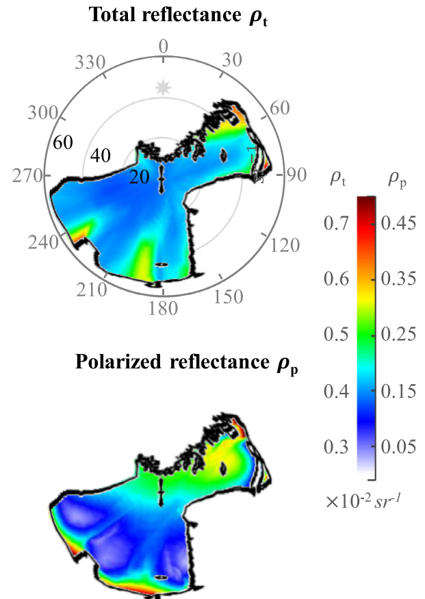
Fig. 14. The estimated total and polarized water-leaving bi-directional reflectances of Case 2 at the 443 nm band as a function of viewing angles.
