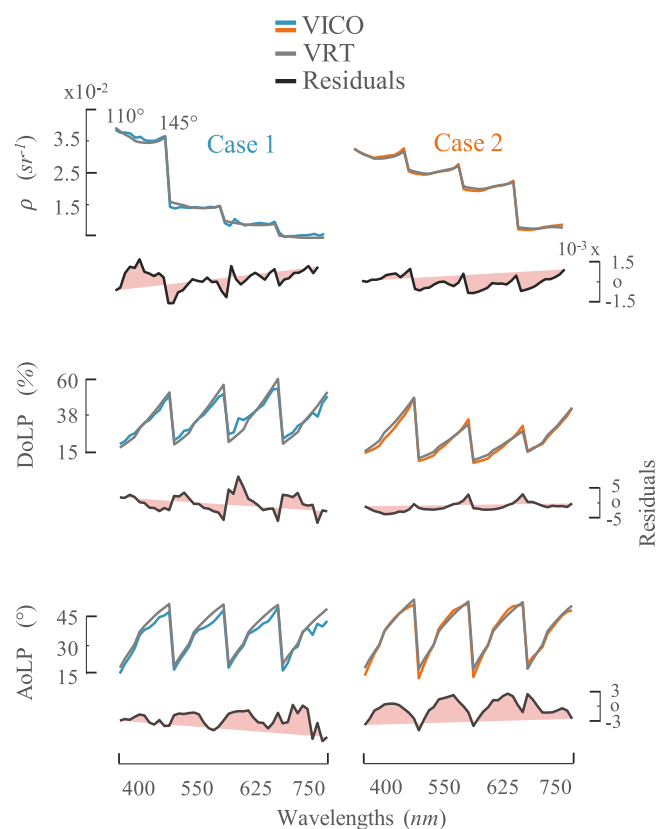
Fig. 8. Multi-spectral, and -angular VRT match with aircraft \rho , DoLP , and AoLP observations for Cases 1 and 2. The matches and residuals (i.e., measurement minus model) of the observed parameters are shown in the left and right-hand axes, respectively. The shaded red areas outline the slope for each of the observed parameter residuals across the spectral bands. Each spectral band is shown as a function of scattering angles. The values of the scattering angle 110° and 145° are indicated for each wavelength. The solar position is at \theta_0 = 44^\circ and \phi_0 = 110^\circ for both cases.
