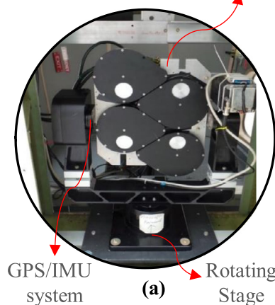
Four cameras with tear drop-shaped filter wheels mounted on a plate
