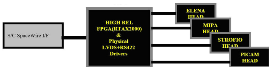
Fig. 40 SCU Architecture
