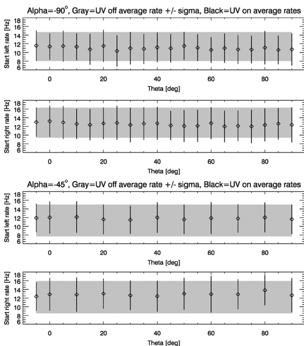
Fig. 63 Results of UV contamination tests for Strofio MCPs
