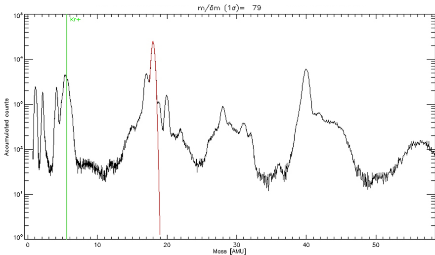
Fig. 56 Strofiu mass range for two turns
