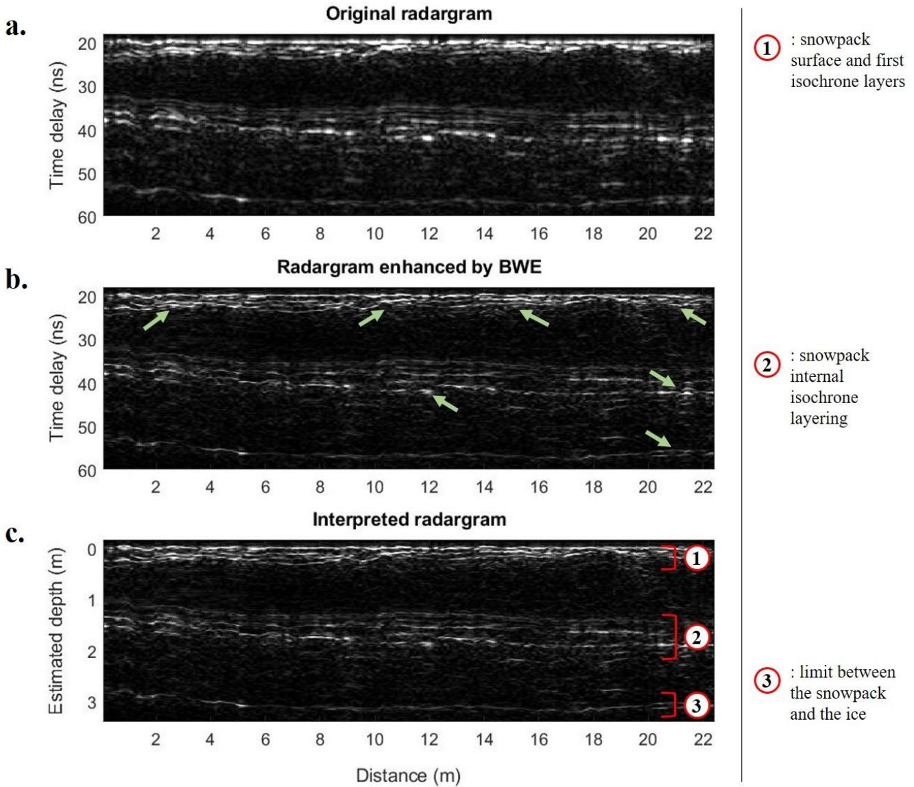
583 584 Figure 17: Radargram from the Chamonix field campaign, before (a) and after (b) application of the BWE. 585 Panel (c) proposes interpretation. The time delays have been converted into distance assuming a dielectric 586 constant of 3.1.
