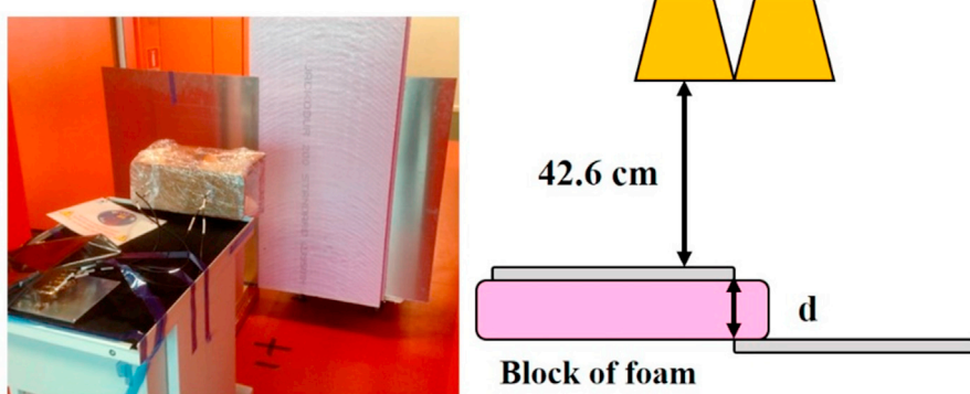
Fig. 9. Illustrations of the experimental set-up for the "two reflectors" experiment performed at LATMOS. a. Experimental set-up without support between the plates b. Experimental set-up with a support between the plate.
