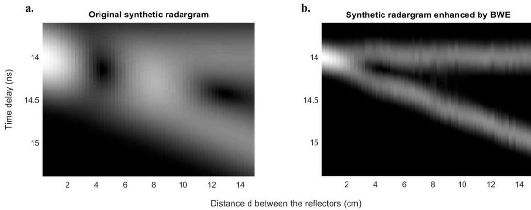
Fig. 2. Synthetic WISDOM radargram generated with two echoes and a white Gaussian noise (SNR = 30 dB) a) without BWE b) with BWE.
