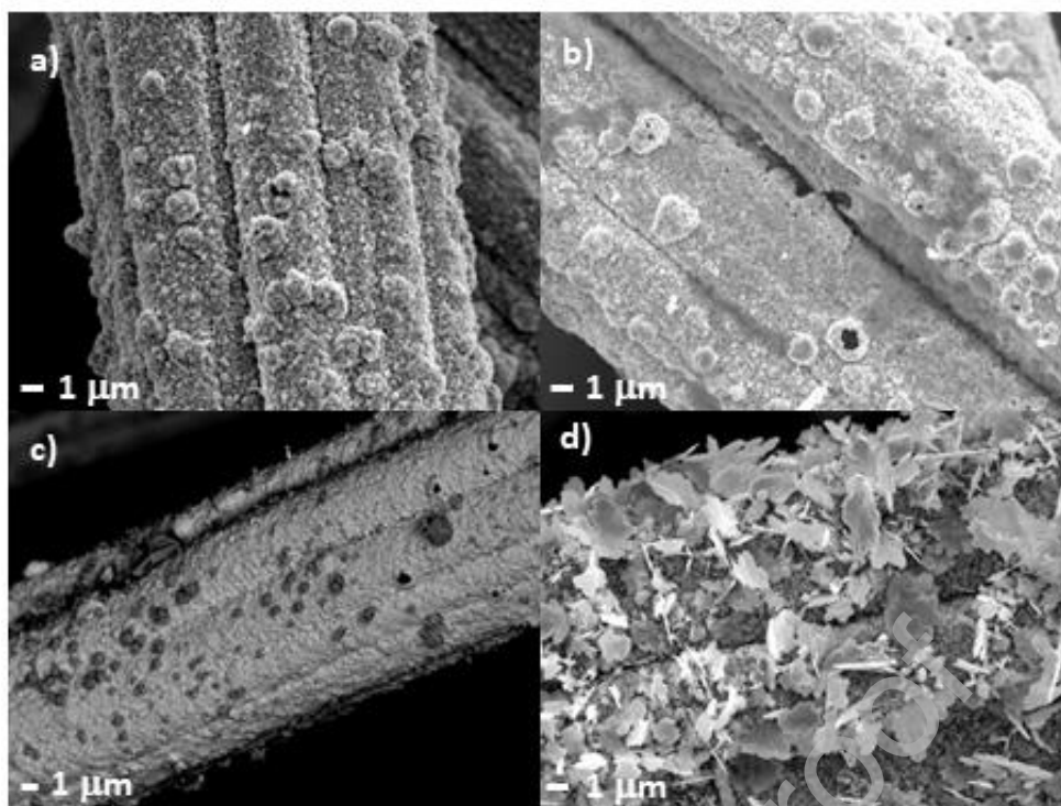
Fig. 2. SEM images of Bi@GF (a,b) and Ag-Bi@GF (c,d) with (b,d) and without (a,c) acid washing and electrochemical pretreatment of Bi@GF. Ag deposition was performed in 2 \text{ mmol L}^{-1} [\text{AgNO}_3] , for 45 min.
