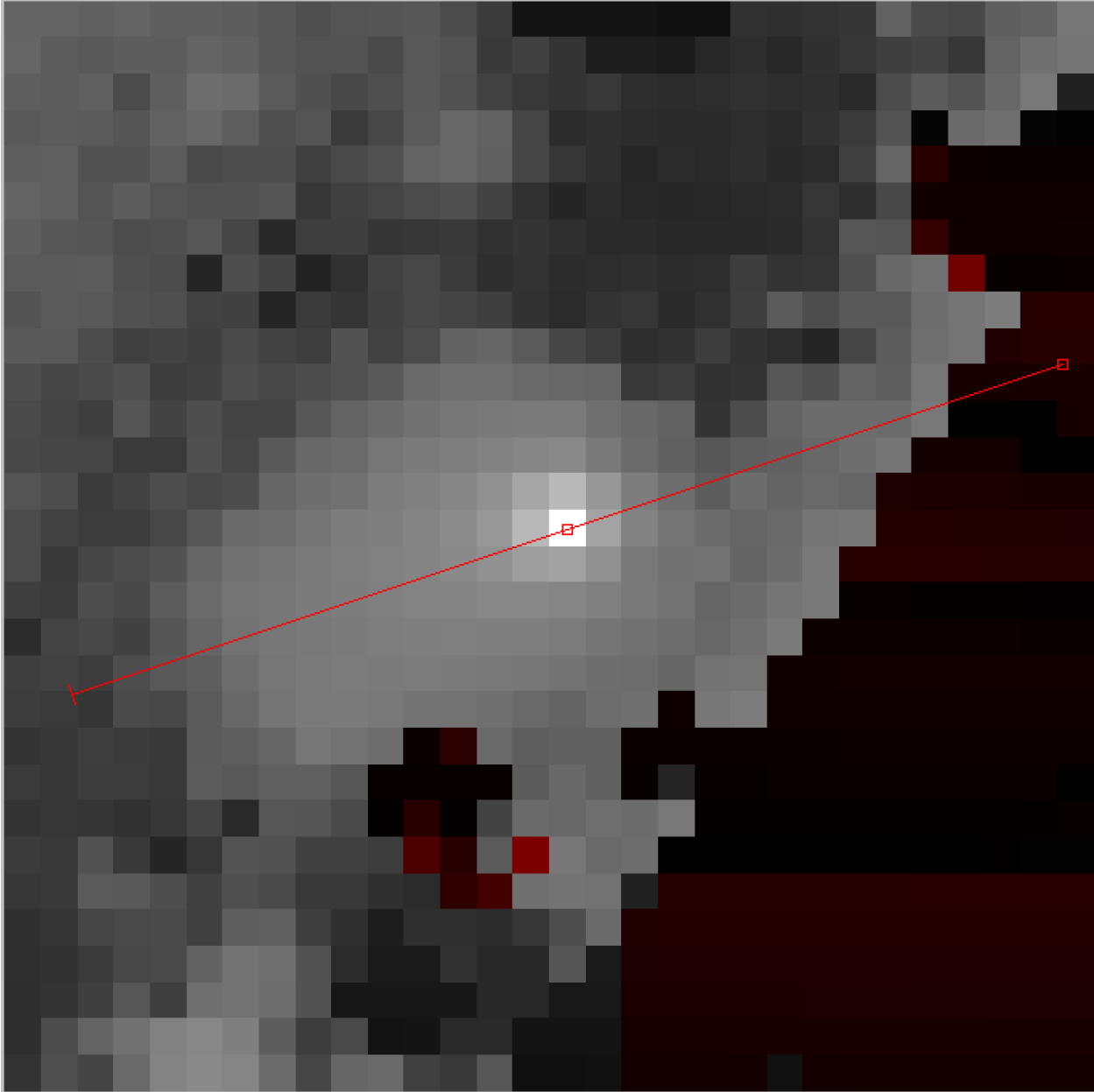
Figure 1. SOHO/SWAN image of the hydrogen coma of comet C/2020 F3 (NEOWISE) observed on 9 July 2020. The field of view is 30^\circ across. The straight line from left to right and slightly upward shows a profile cut along the maximum extent of the hydrogen "tail" whose profile is shown in Figure 2. The dark region toward the right and lower right corresponds to the solar avoidance area of SWAN with the direction to the to the right Sun.
