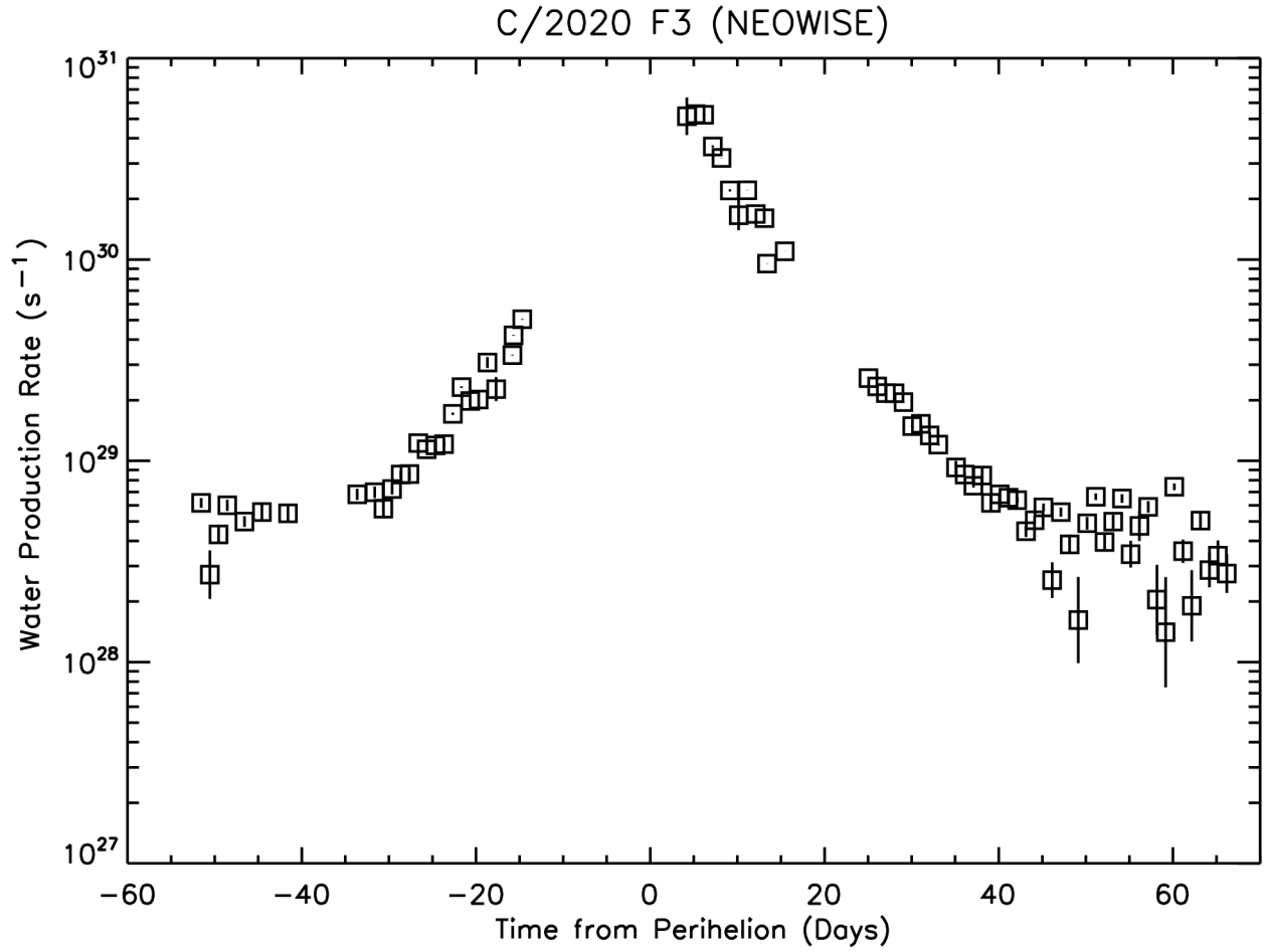
Figure 3. Water production rate in comet C/2020 F3 (NEOWISE) plotted as a function of time in days from perihelion. The error bars indicate the 1-\sigma uncertainties resulting from noise in the data and the fitting of the coma model and interstellar background.
