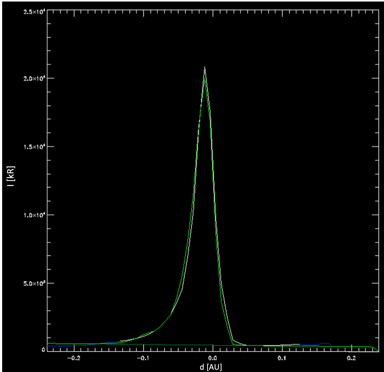
Figure 2. Model-Data comparison profile along the long extent of the hydrogen “tail” of comet C/2020 F3 (NEOWISE) observed by SOHO/SWAN on 9 July 2020. The white curved line corresponds to the observed brightness along the cut shown in Figure 1 along the maximum extent of the hydrogen tail. The flat straight green line near the bottom corresponds to the fitted interstellar hydrogen background. The curved green line is the fit of the coma model to the observed image. The red line toward the lower right is where the observed profile cuts through a field star that has been marked to be ignored. Note that the shape of the model profile follows the asymmetric coma distribution that is produced by radiation pressure from the resonance scattering of the
