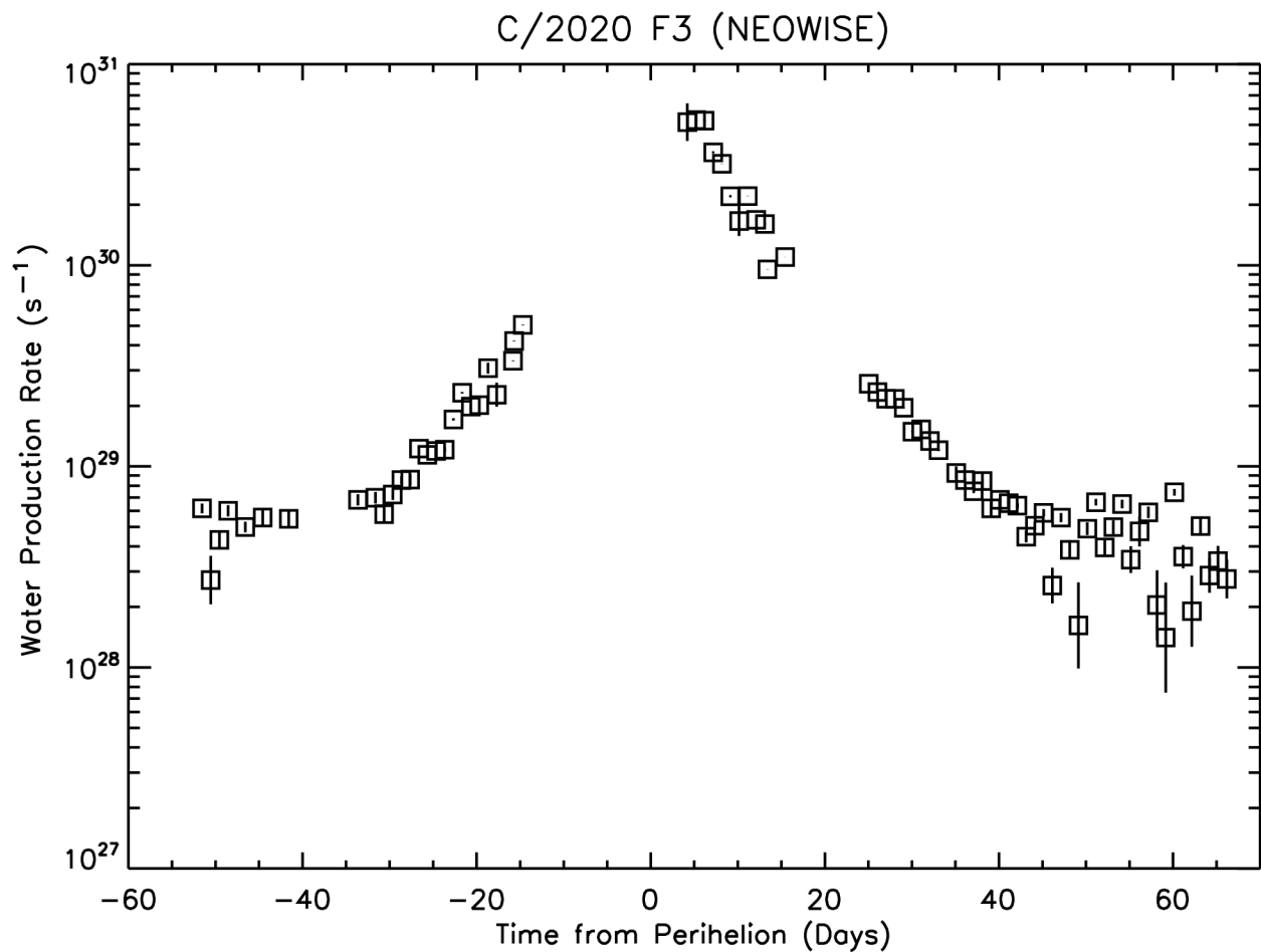
Figure 3. Water production rate in comet C/2020 F3 (NEOWISE) plotted as a function of time in days from perihelion. The error bars indicate the 1\text{-}\sigma uncertainties resulting from noise in the data and the fitting of the coma model and interstellar background.
