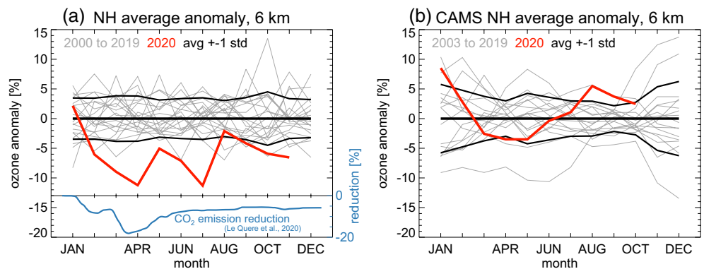
Figure 2. Annual cycles of monthly mean northern extratropical ozone anomalies at 6 km altitude. Anomalies are in percent, relative to the climatological monthly mean calculated for each station/instrument, and for the period 2000–2020 (all Januaries, all Februaries, ..., all Decembers). These single station/instrument anomalies are then averaged over all northern extratropical stations/instruments (north of 15°N). Panel (a) Results from the station observations. Panel (b) Results for CAMS atmospheric composition (re-)analyses at grid points nearest the stations. The CAMS data do not account for COVID-19 related emissions reductions in 2020. Gray lines: individual years from 2000 to 2019. Thick red line: year 2020. Thick black lines: average anomaly, \pm 1 standard deviation over the years. Dark blue lines and scale on the right in panel (a): Global CO 2 emission reduction in 2020 (in percent) from Le Quéré et al. (2020b), as in Figure 1. CAMS, Copernicus Atmosphere Monitoring Service.
