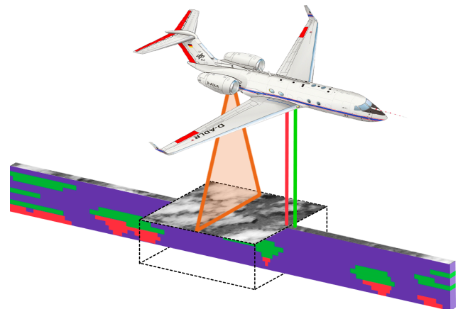
Figure 2. Combined lidar (WALES), radar (HAMP MIRA), and solar radiance measurements (specMACS) from the German High Altitude Long Range Research Aircraft ( HALO ). Lidar (green) and radar (red) provide along-track cross-sections through the atmosphere, while the swath of the imager (orange) captures the across-track dimension of the scene.
