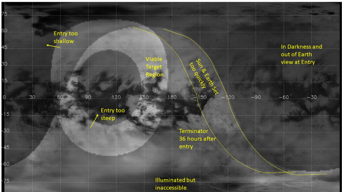
Figure 2. Schematic illustration of the combined delivery constraints. Given the incoming direction on a given epoch, the aerodynamic/aerothermodynamic constraints define a toroidal region where the flight path angle is in an allowable range. To perform descent while in Earth communication and with illumination requires being on the dayside at entry. Requiring a period of some days on the ground before sunset eliminates the late afternoon sliver of the daylight region. The logical AND combination of the entry and illumination constraints defines the accessible region for that entry epoch. The accessible regions for a range of arrival epochs (defined by the allowable Titan-relative entry velocity) can be combined in a logical OR sense to yield the ultimate set of possible target locations.
