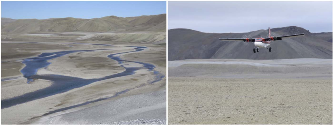
Figure 14. Field photographs from the Haughton impact structure. Although steep slopes exist, flat areas of sand and gravel permit even fixed-wing aircraft to find landing sites. (Photos: Neish).
