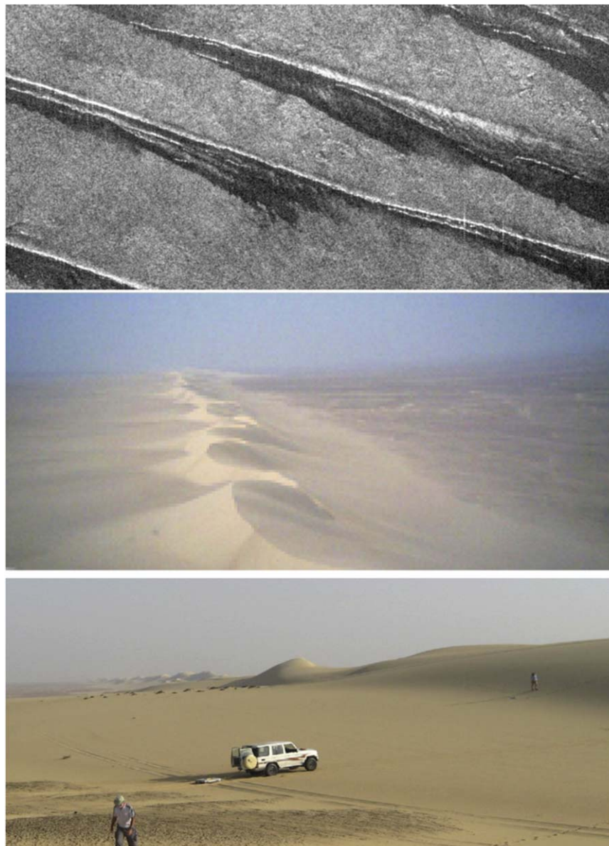
Figure 13. (Top) Tapering linear dunes in Egypt, morphologically identical in radar images (XSAR) with the dunes seen to the Southeast of Selk. (Middle) Kiteborne camera view of Ghard el Quattaniya linear dunes west of Cairo, Egypt showing dune and plinth. (Bottom) Field photo at same dune showing Ground Penetrating Radar operations. While dune slopes themselves would be avoided, it is clear that shallow-sloped dune plinths can allow safe access to sand material. (Photos: Lorenz).
