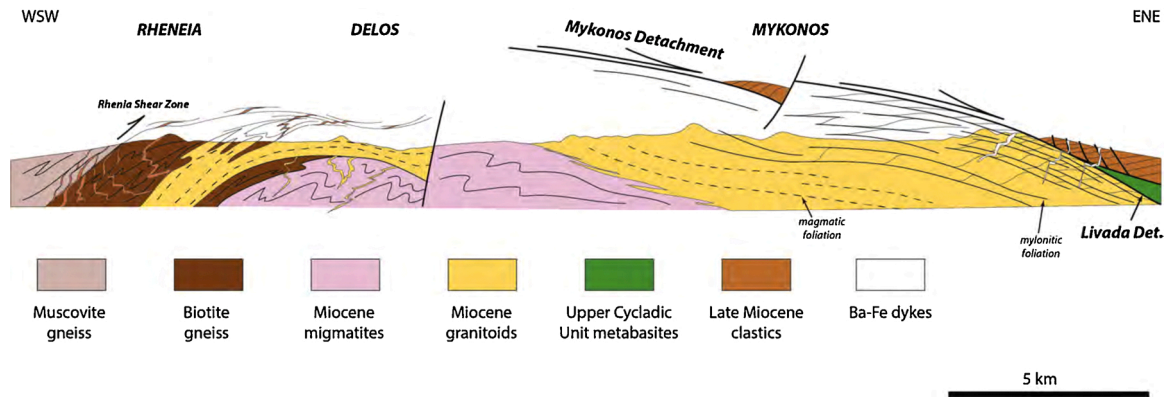
Fig. 11. Synthetic cross-section through Rheneia, Delos and Mykonos, from the migmatitic core to the supra-detachment basin. No vertical exaggeration.
