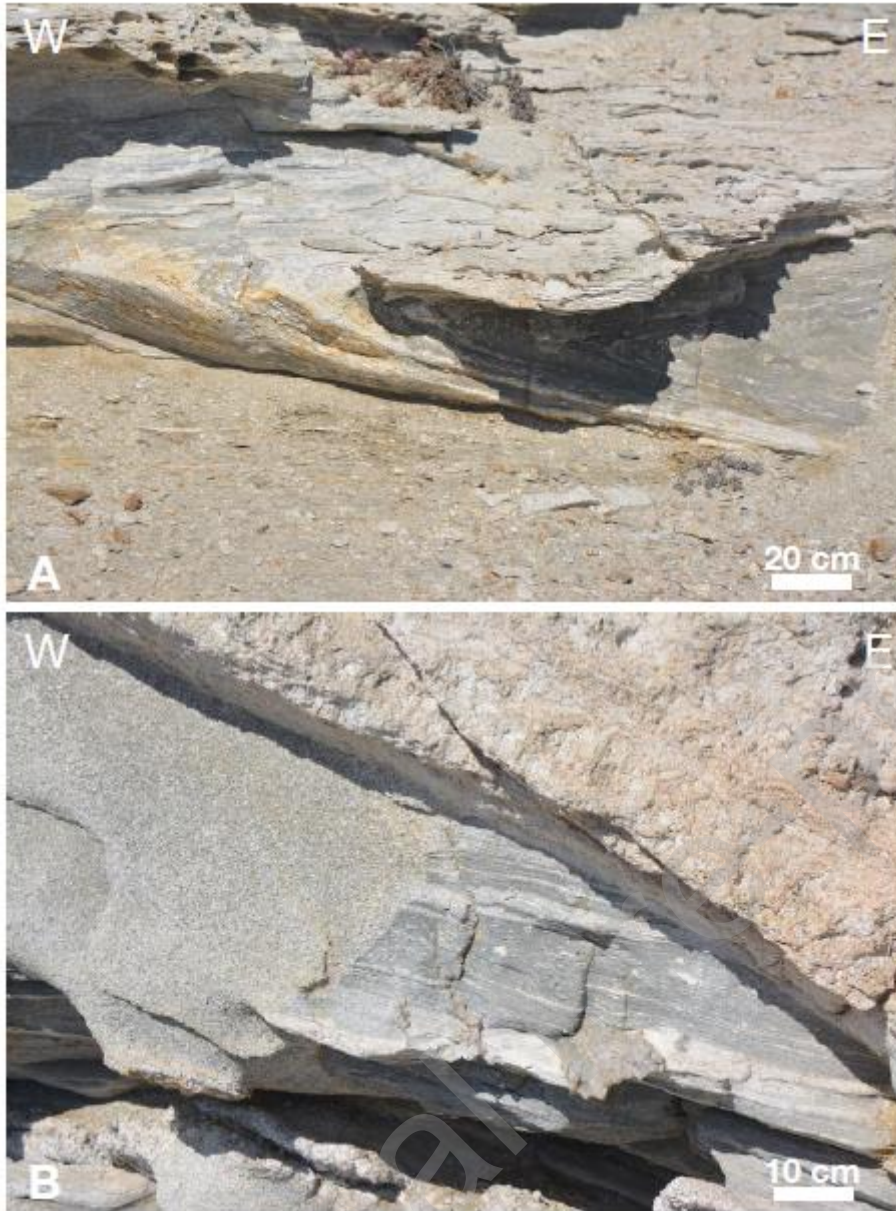
Figure 8: Progressive deformation of dykes within the Rheneia Shear Zone on Rheneia. A: Syn-folial folds affecting already transposed dykes. B: three generations of dykes with different grain size in the YZ plane. All three generations show stretching in the perpendicular direction. Location on figure S0.
