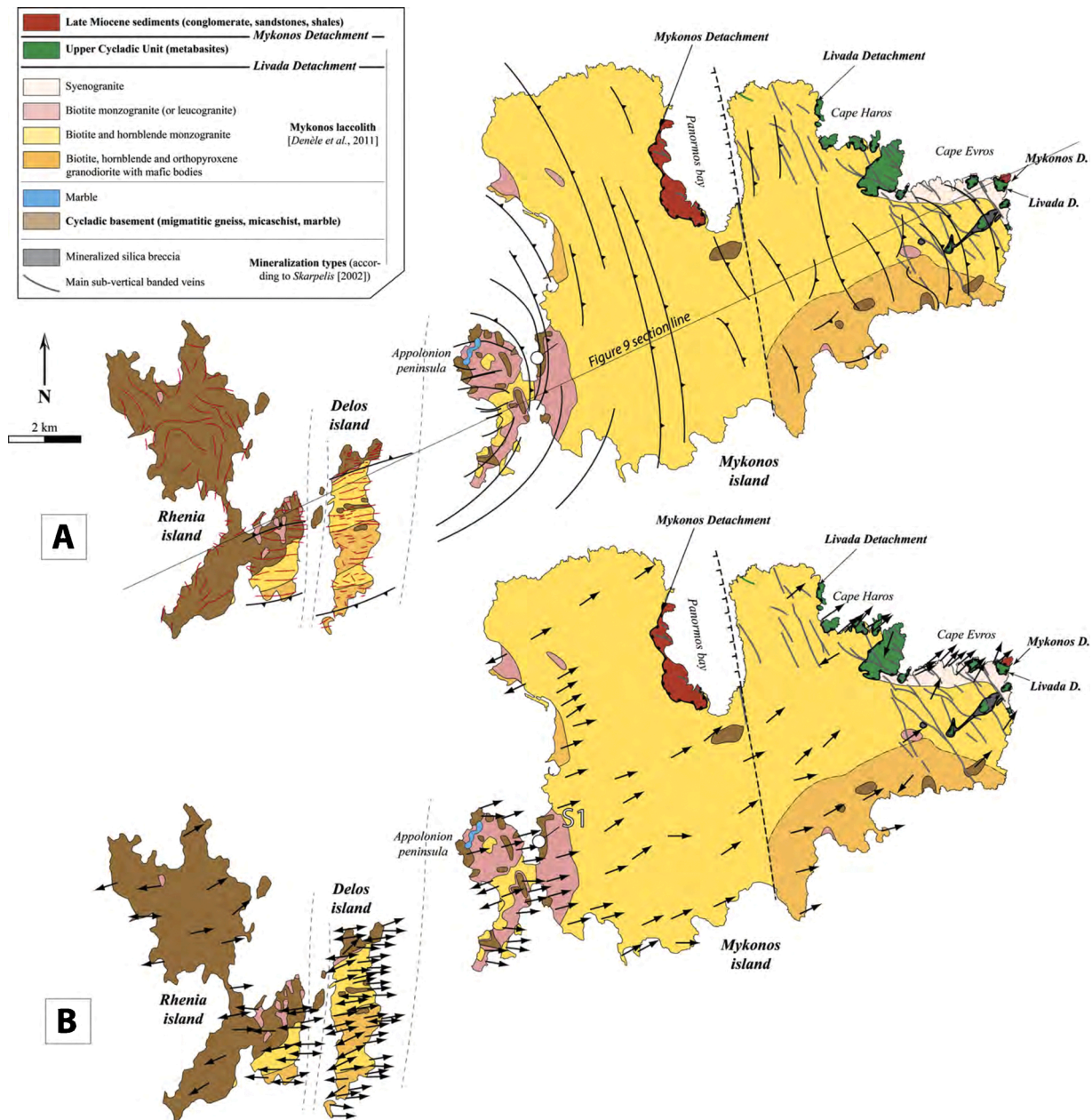
Fig. 3. Tectonic map of the Mykonos-Delos-Rheneia metamorphic core complex. A: foliation trajectories, B: stretching lineations. Compiled after Lucas (1999); Denèle et al. (2011) and Menant et al. (2013).
