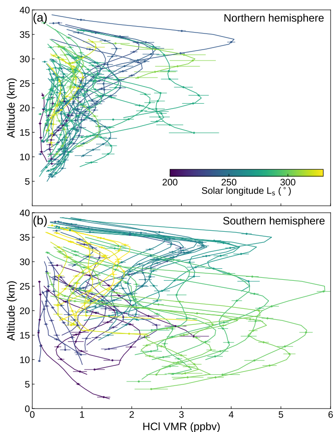
Fig. 3. Retrieved vertical profiles of HCl during the Mars year 35 dust season. The mean retrieved HCl VMR vertical profiles for each occultation made in a : the northern hemisphere, and b : the southern hemisphere during Mars year 35. Colours indicate solar longitude, L_s .
