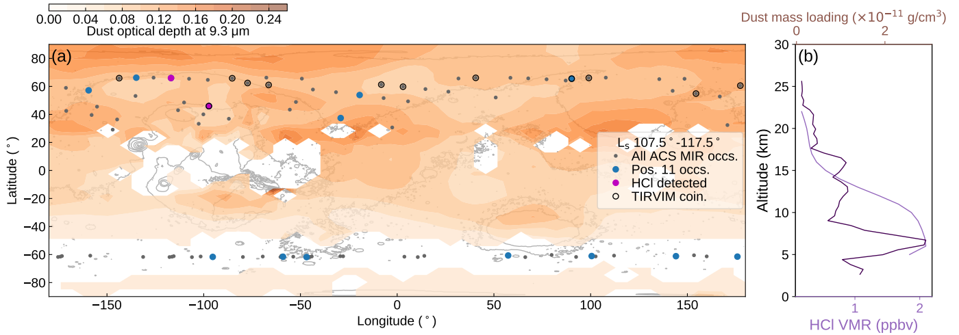
Fig. A8. Panel a shows the spatial distribution of dust optical depth at 9.3 \mu\text{m} Montabone et al. (2020) averaged between L_s = 107.5\text{--}117.5^\circ over a map of Mars. Also shown are the tangent point locations of ACS MIR solar occultations. Highlighted are occultations made using position 11, those in which HCl was observed, and those with coincident TIRVIM observation (northern only). Panel b shows the vertical profiles of HCl VMR from ACS MIR and dust mass loading from ACS TIRVIM Luginin et al. (2020) for the coincident observation at ( 46^\circ\text{N} , 97^\circ\text{W} ).
