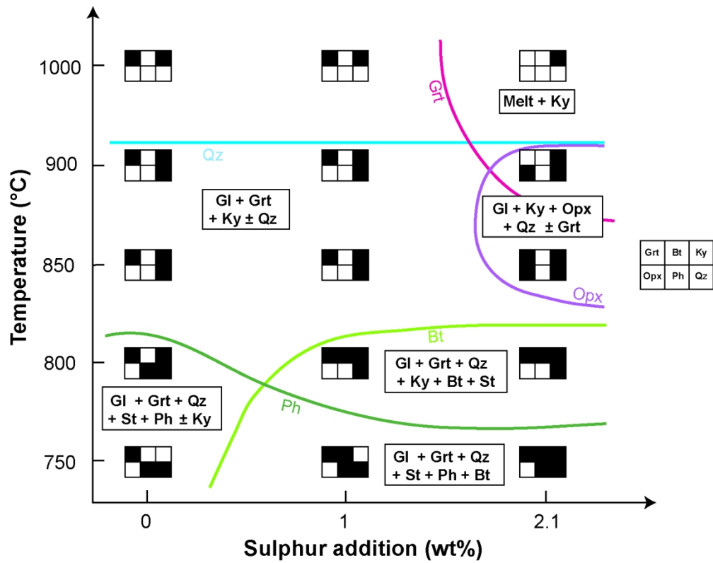
Fig. 4: T-wt. % S_{in} stability fields of different parageneses of the main minerals in subducted Ca-poor pelite. The approximate stability limits of key phases are indicated; the curves are labelled with mineral lying inside their respective stability fields. Abbreviations as in Fig. 2 + Ph = phengite and Gl = glass.
