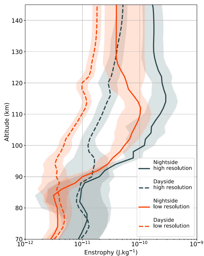
Fig. 9. Eddy entrophy as a function of altitude averaged over 1 Vd and latitude lower than 75^\circ , on the day and night sides, at high ( 96 \times 96 ) and low ( 48 \times 32 ) resolutions. The envelopes show the minima and maxima for 1 Vd.
