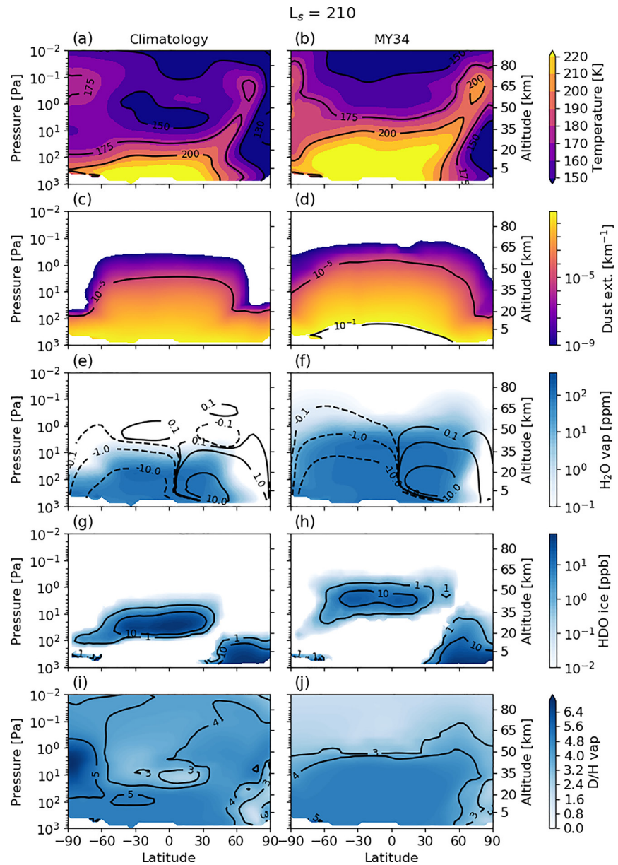
Figure 3. Zonally averaged meridional profiles of (from top to bottom) temperature (a) and (b), dust extinction at 500 nm (c and d), \text{H}_2\text{O} vapor (e and f), HDO ice (g and h) and D/H ratio of the vapor (i and j), at a local-time of 14 h and at solar longitude L_s = 210^\circ . The left column is the Climatology scenario and the right column is MY34. The contours on panels (e and f) are the zonally averaged stream function (in units of 10^9 kg/s), with positive values indicating a clockwise circulation.
