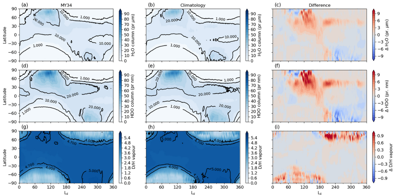
Figure 2. Seasonal evolution of the zonally averaged column of \text{H}_2\text{O} (a and b) and HDO (d and e) in the vapor phase, for the climatology and Martian year 34 (MY34) scenarios. Below is the corresponding D/H ratios in terms of standard mean ocean water (SMOW) (g and h), for the vapor phases. Units are precipitable microns or nanometers. Left column is for MY34, center column for the climatology scenario and right column (c, f, and i) is the absolute difference between MY34 and climatology. A similar figure for the ice phase can be found in the supplementary information.
