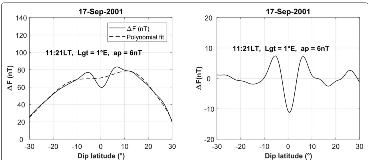
Fig. 3 The magnetic signature of the equatorial electrojet (EEJ). The left panel shows the total residuals \Delta F (solid line) and background long wave length signal (dashed line). The right panel shows the EEJ magnetic signature isolated from the total residuals
