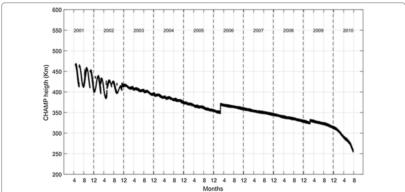
Fig. 4 CHAMP satellite altitude variations from 2001 to 2010
