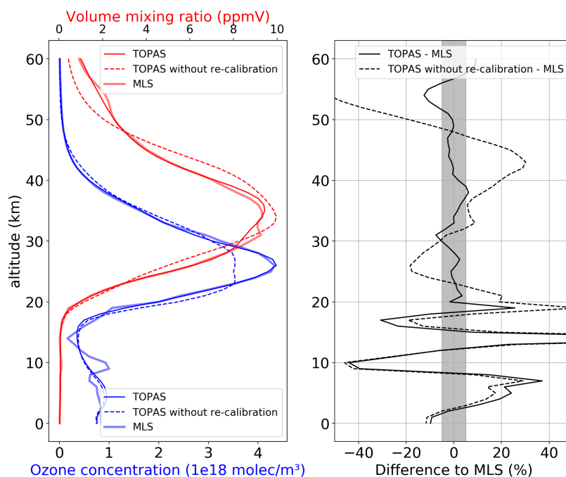
Figure 6. Comparison of ozone profiles from the TOPAS retrieval with MLS data for a single TROPOMI pixel (6 April 2019, orbit nr. 7664, 16.15^\circ latitude, -23.53^\circ longitude, SZA: 20.15^\circ , VA: 11.47^\circ and RAZ 6.60^\circ ). Results for the TOPAS retrievals with and without calibration correction are shown. Left: Ozone concentration (blue) and volume mixing ratio (red) from TOPAS/TROPOMI and the collocated MLS measurement. Right: Relative differences between TOPAS retrieval and MLS. The relative differences are identical for both ozone concentration (blue) and volume mixing ratio (red).
