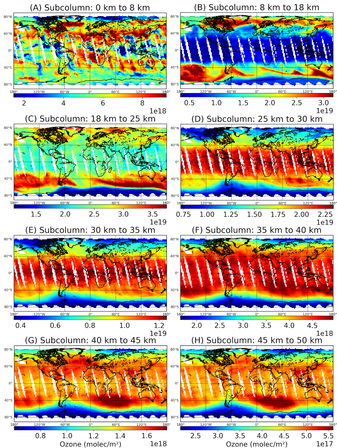
Figure 11. TROPOMI ozone subcolumns for selected atmospheric layers for 1 October 2018. Vertical thicknesses of the layers roughly approximate the vertical resolution of the ozone profiles.
