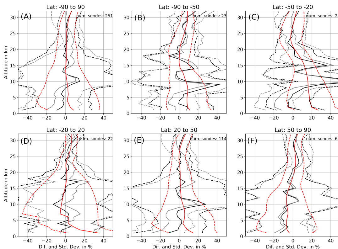
Figure 7. Comparison of the ozone profiles retrieved from TROPOMI and those from ozone sondes for different zonal bands. The relative mean difference between the retrieval results and the high resolution sonde data (solid line) as well as the standard deviation of the differences (dashed line) are shown in black. The comparison with the sonde profiles convolved with the TOPAS averaging kernels is shown in red. In grey the relative difference between the a-priori ozone profiles and high resolution ozone sonde profiles are displayed along with the corresponding standard deviations.
