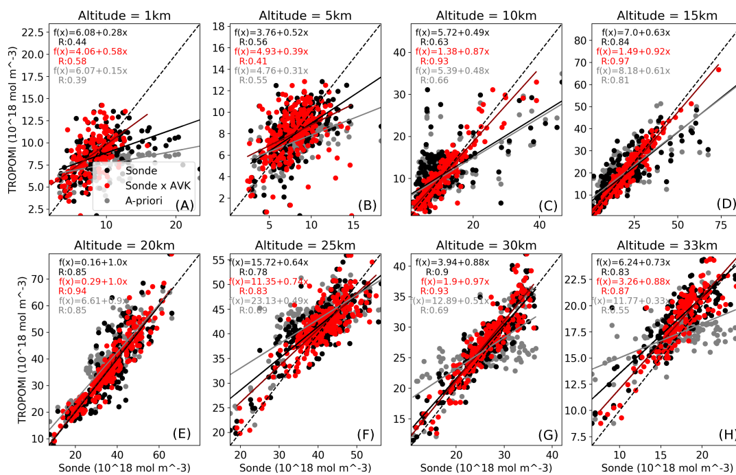
Figure 8. Scatter plot of collocated TROPOMI and ozone sonde profiles, the latter with and without convolving with TOPAS averaging kernels (red and black, respectively) for different altitudes. The comparison between a-priori and sonde profiles is shown in grey. The solid lines show the linear fit. The R-value is indicated in the top left corner of each panel (also black and red). The ideal 1:1 curve is plotted as a dashed line.
