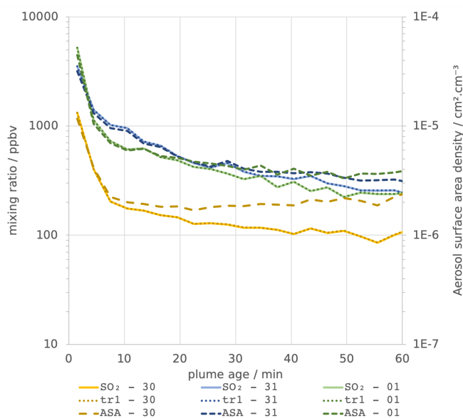
Figure 6. Modelled average in-plume mixing ratios of, on left axis, \text{SO}_2 (solid lines) and tracer1 (tr1, dotted lines) and, on right axis, density of aerosol surface area (ASA, dashed lines). Note that both y-axes are logarithmic.
