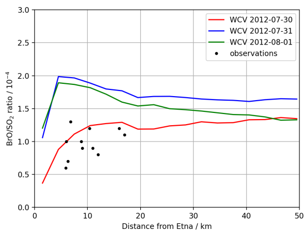
Figure 12. Modelled BrO/SO 2 ratio at 1200 UTC on 2012-07-30, 2012-07-31, and 2012-08-01 (lines), and observed BrO/SO 2 ratios for 2012-07-24 – 2012-08-02 (Surl et al., 2015) (circles), plotted against distance from the volcano. We caution that these observations, taken over several days with varying wind speeds, should not be interpreted as representing temporal evolution.
