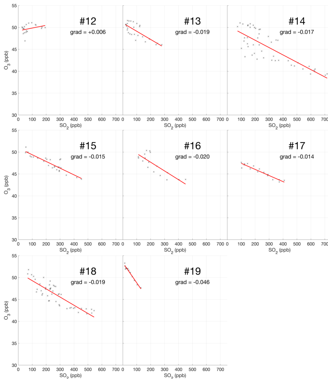
Figure 5. Measurements of SO 2 and O 3 mixing ratios for the eight major plume encounters on 1 August 2012.
