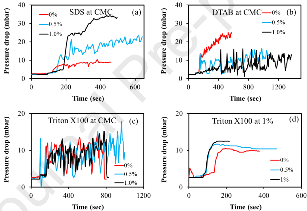
Figure 6: Measured pressure drop versus time during foam injection at different experimental conditions in the Hele-Shaw cell. The legends indicate nanoparticle concentrations.
