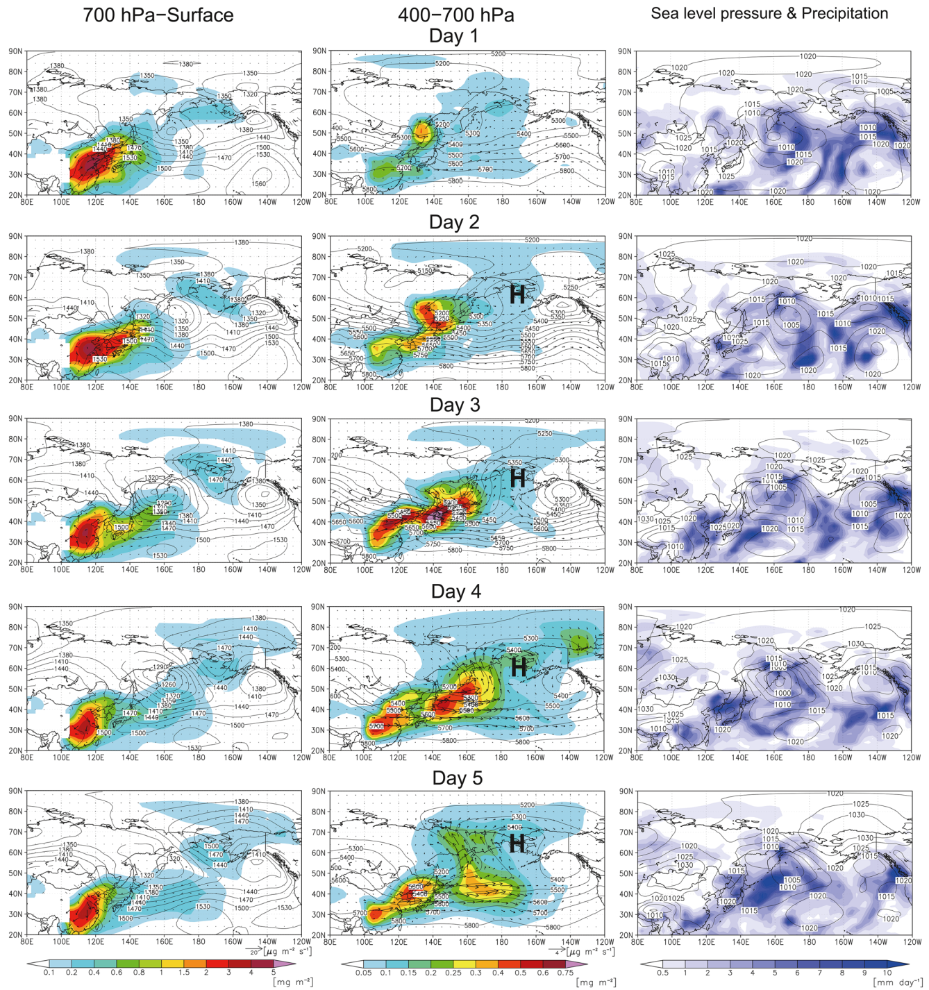
Figure 8. Composited black carbon (BC) column, horizontal BC fluxes, and geopotential height in the lower and middle troposphere for six events of the Pacific route. H indicates the location of the high-pressure center.
