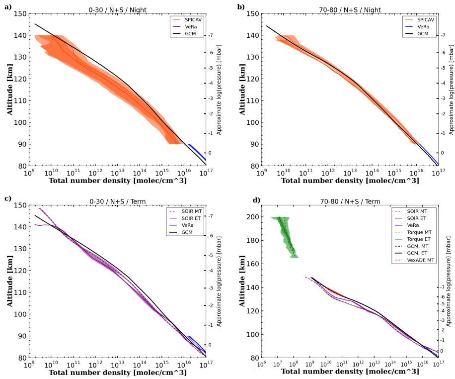
Figure 6: Measured total density profiles (molecule/cm 3 ) retrieved with different Venus Express instruments at nighttime (Panels a and b) and at the terminators (Panels c and d) for two latitude bins 0-30° and 70°-80° (North/South averages) as indicated. The colored areas mark the uncertainty of the respective averaged profiles at one standard deviation. The figures are adapted from Figures 20 and 23 in Limaye et al. (2017). Model predictions averaged at same latitudes and local time as observations are plotted with solid and dashed black lines. Vertical axis is given in altitudes, and approximate pressure (in mbar) is shown as the right hand side vertical axis.
