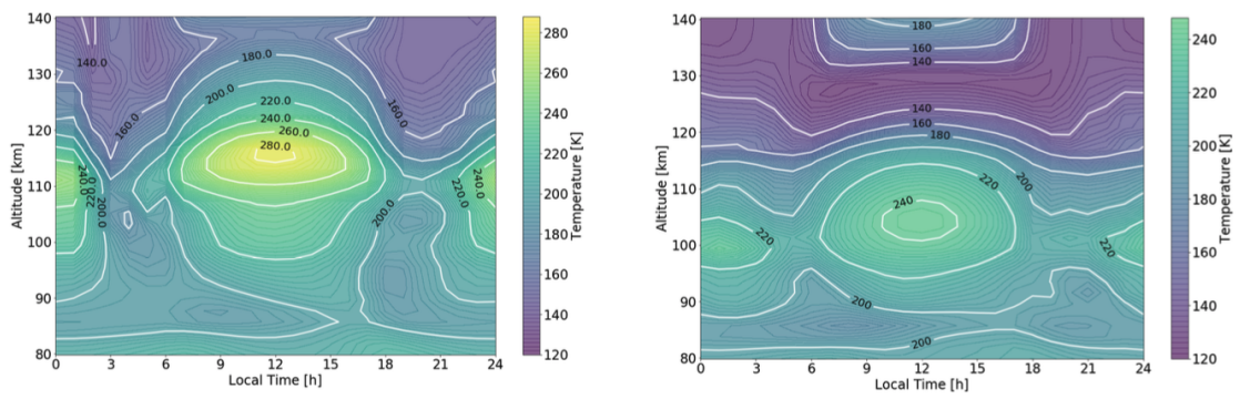
Figure 2: Temperature field (local time versus altitude) obtained with IPSL-VGCM before (left panel) and after (right panel) the non-LTE parameterization improvements, listed in Table 1.
