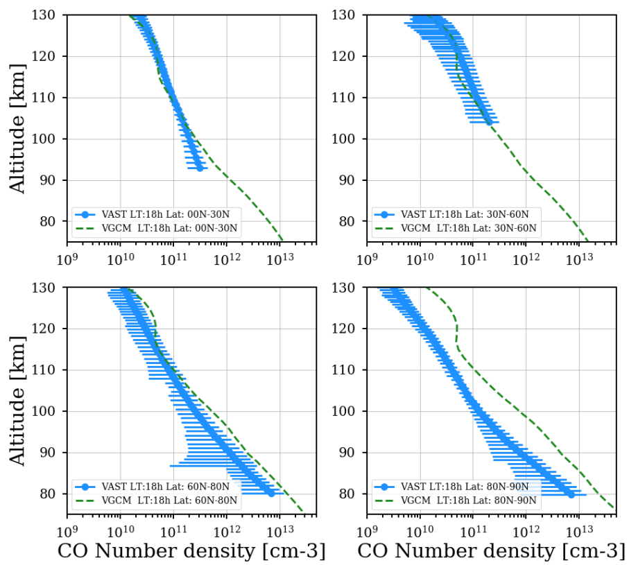
Figure 10: Same as Figure 9 but for evening terminator (ET), LT = 18h
