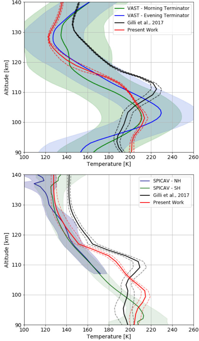
Figure 1: Averaged temperature vertical profiles as function of altitude predicted by the IPSL-VGCM before (solid black line) and after (solid red line) improving the non-LTE parameterization, together with observational data from Venus Express. Top panel: temperature retrieval results at the terminator (green for morning and blue for evening terminator) at the latitude bin 30^{\circ}\text{N} - 60^{\circ}\text{N} extracted from the Venus Atmosphere from SOIR data at the Terminator (VAST) database (Mahieux et al., 2015). SOIR standard deviation is also plotted as shaded green and blue areas. Bottom panel: Temperature retrieval results from SPICAV/VEx for the Northern Hemisphere (SPICAV - NH), 30^{\circ}\text{N} - 50^{\circ}\text{N} in dark blue, and for the Southern Hemisphere (SPICAV - SH), 30^{\circ}\text{S} - 50^{\circ}\text{S} in green (after Piccialli et al. (2015)). Standard deviation of the predicted temperature mean, in the same local time and latitude range as observed, is represented by dashed lines.
