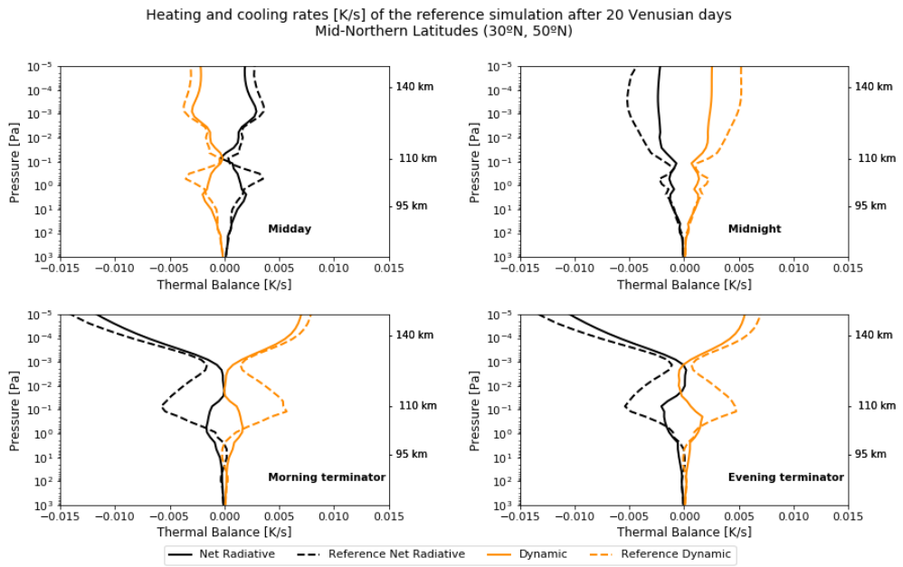
Figure B.18: Net radiative and dynamical rates [K/s] obtained in this work for mid northern latitudes (30°N-50°N) after improving the Non-LTE parameterization for midday, nighttime and terminators, as indicated in the panels. For comparison, the rates obtained in a previous version of the IPSL-VGCM (Gilli17), labeled as “reference”, are also shown. Approximate altitudes are indicated on the right side of the panels.
