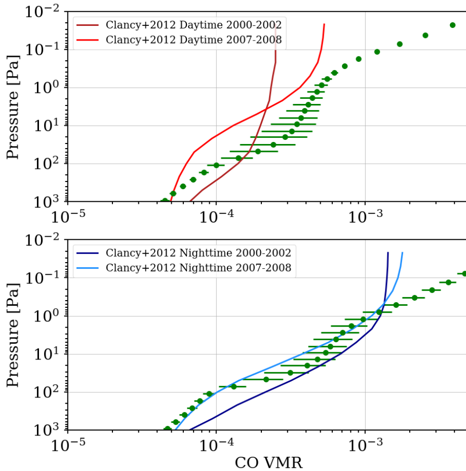
Figure 8: IPSL-VGCM CO volume mixing ratio profiles (green dots) as function of pressure, averaged in latitude bin 60^{\circ}\text{N} - 60^{\circ}\text{S} , 10h-14h LT for daytime and 22h-2h for nighttime, with variability indicated as standard deviation of the average. CO profiles retrieved from sub-mm CO absorption line observations as in Clancy et al. (2012) for daytime (top panel) and nighttime (bottom panel) are also plotted. 2000-2002 disk average daytime/nighttime measurements are in dark red/blue solid lines, while 2007-2008 disk average daytime/nighttime measurements are in red/blue solid line.
