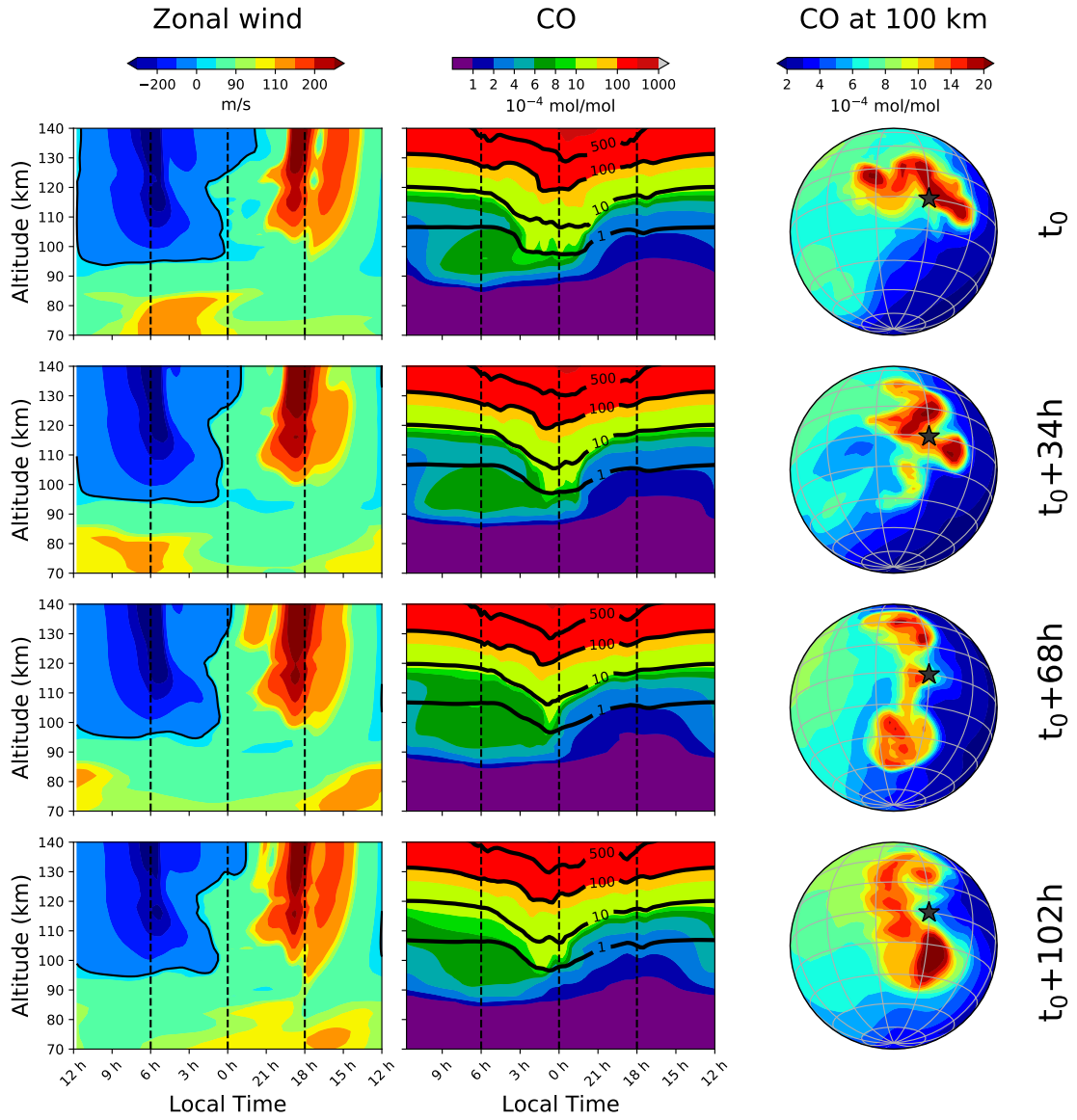
Figure 16: Four consecutive snapshots, from left to right, of: (1) 2D local time vs. altitude map of zonal wind averaged for latitudes 20^{\circ}\text{S} - 20^{\circ}\text{N} , (2) 2D local time vs. altitude map of CO vmr [mol/mol] averaged for latitudes 20^{\circ}\text{S} - 20^{\circ}\text{N} (3) 3D map of CO vmr [mol/mol] at 100 km, the AS point is indicated by a black star.
