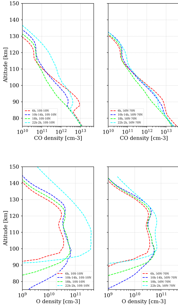
Figure 14: Local time variations of IPSL-VGCM CO (top panels) and O (bottom panels) density profiles at equatorial regions 10S-10N (left panels) and middle-high latitudes 50N-70N (right panels). Daytime and nighttime profiles are averaged between LT=10h-14h and LT=22h-2h, respectively. Evening (18h) and morning (6h) terminators are also plotted.
