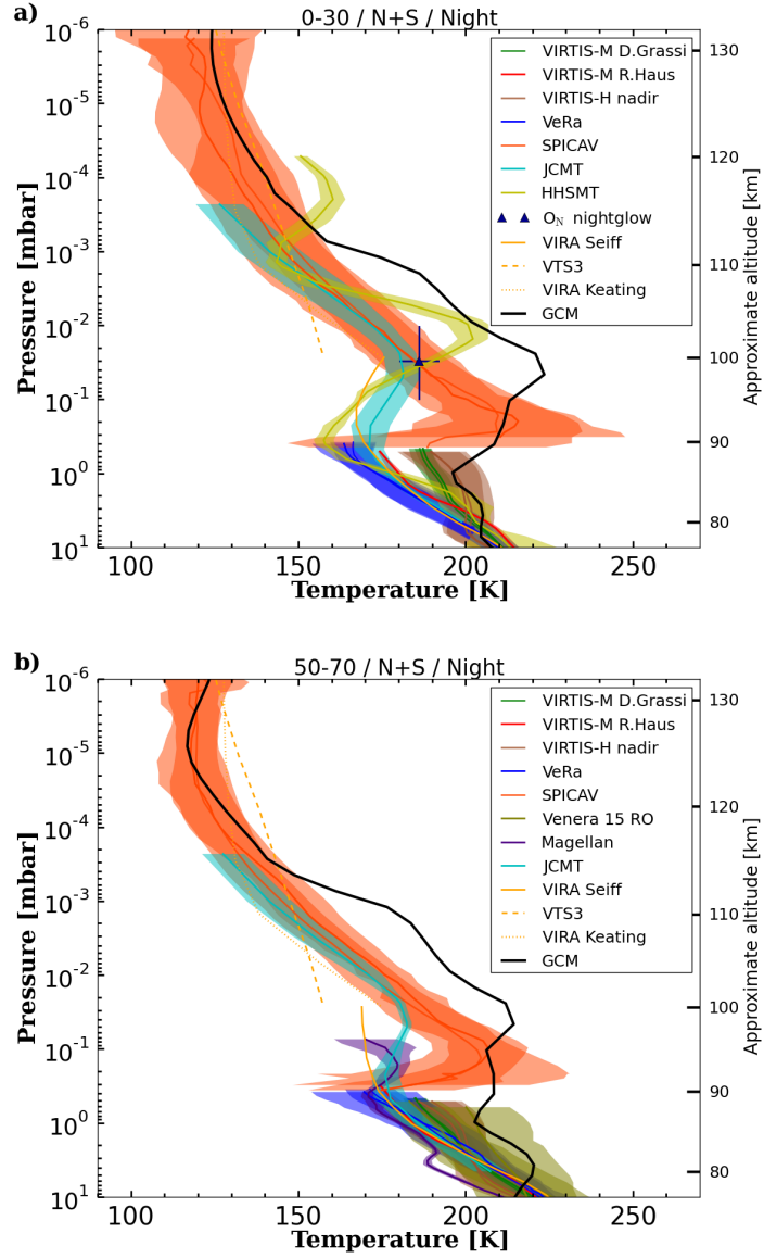
Figure 3: Compilation of available nighttime Venus temperature profiles above 80 km both from spacecrafts and ground based telescopes versus model predictions averaged at equatorial latitudes 0-30^\circ from Southern and Northern hemispheres (top panel) and 50^\circ-70^\circ N/S (bottom panel). Corresponding approximate values for altitude is given on the right hand side of the panel. Panel a) and panel b) are adapted from Figure 15 and 17 in Limaye et al. (2017), respectively. See text for details. Uncertainties (one standard deviation) are either plotted as colored areas for averaged profiles in the same bin (Venus Express datasets, JCMT, HHSMT) or as error bars ( O_2 nightglow). The IPSL-VGCM predicted profile is plotted with solid black line.
