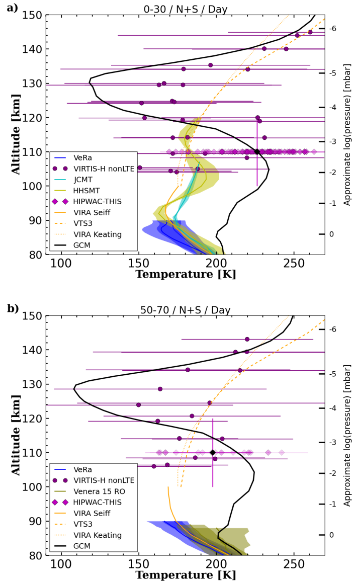
Figure 5: Same as Figure 3 but for daytime and with the addition of temperature retrieved from CO non-LTE emissions observed by VIRTIS/VEx. See text for details. Panel a) and panel b) are adapted from Figure 15 and 17 in Limaye et al. (2017), respectively.
