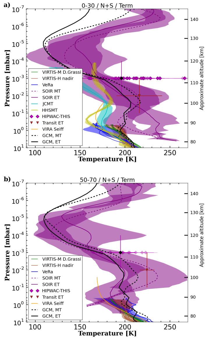
Figure 4: Same as Figure 3 but at the terminators (morning and evening) and with the addition of the mean temperature values retrieved at the evening terminator during the Venus transit in 2012. See text for details. Panel a) and panel b) are adapted from Figure 15 and 17 in Limaye et al. (2017), respectively. The IPSL-VGCM predicted profiles are in solid and dashed black lines for the ET and MT, respectively.
