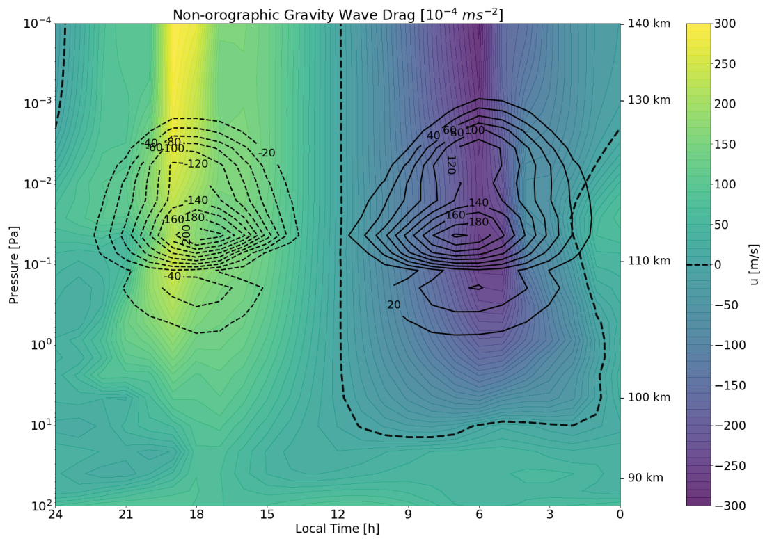
Figure 17: Local time-pressure distribution of the GW zonal drag (contours) integrated over all latitudes ( \theta ) and normalized by \cos(\theta) to account for conservation of angular momentum. Zonal winds (color) at equator regions ( 10^\circ\text{S} - 10^\circ\text{N} ) are also shown. Solid line indicates acceleration, dotted line deceleration. Positive zonal wind values are westward and negative zonal wind values are eastward. Dashed-line indicates the region where the zonal wind converges to zero.
