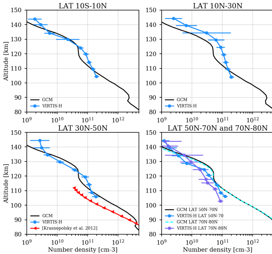
Figure 7: CO density retrieved by VIRTIS/VE x during daytime (LT 10h-14h) after Gilli et al. (2015) together with IPSL-VGCM averaged profiles binned at similar latitude and local time, as indicated in the panels. In addition, semi-empirical CO profile from Krasnopolsky (2012) representative of mean conditions is shown for comparison with mid-latitude (30°N-50°N) daytime averaged profiles.
