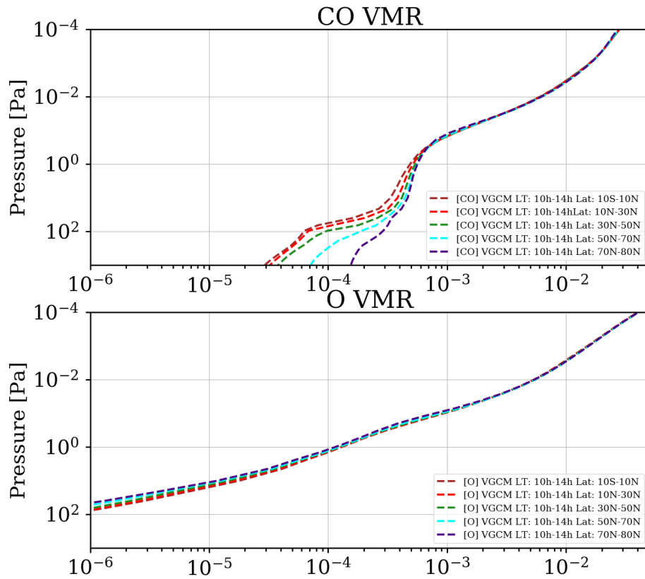
Figure 12: Latitudinal variations of CO and O vmr during daytime (10h-14h) predicted by the IPSL-VGCM. The latitude bins are indicated in each panel. The pressure levels correspond to an altitude range between 75 and 140 km, approximately. CO profiles show a clear transition of regime at around 1 Pa (100-110 km)
