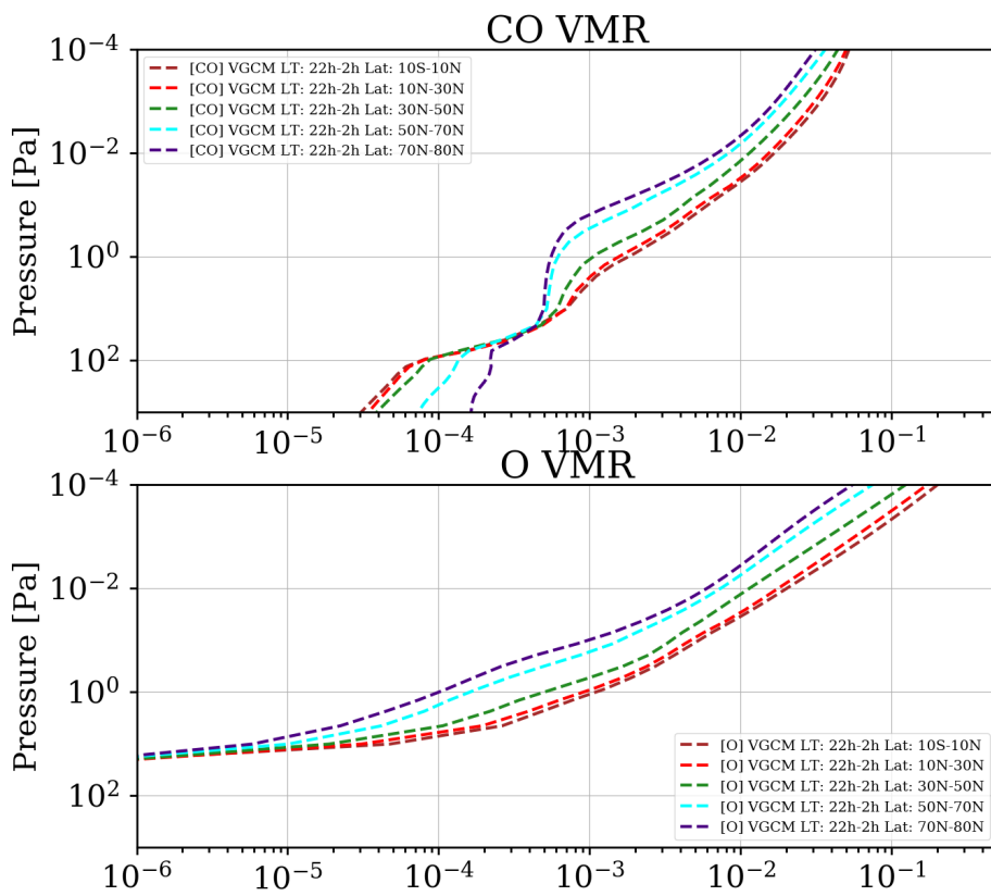
Figure 13: Latitudinal variations of CO and O vmr during nighttime predicted by the IPSL-VGCM. The latitude bins are indicated in each panel.
