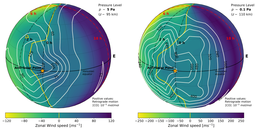
Figure 15: 3D maps of Venus nightside at 5 Pa (left) and 0.1 Pa (right) averaged for one Venus solar day, the anti-solar point is indicated with a star. Contour white lines: CO vmr and colors are zonal wind fields. Yellow lines indicate where the horizontal wind converges to zero values. The location of the terminator is represented by red dashed lines.
