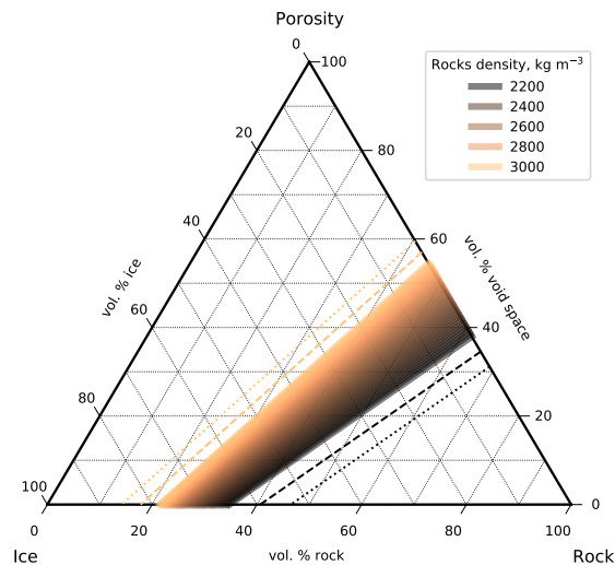
Fig. 3: Bulk composition of Sylvia, assuming three end members: rocks, ices (density of 920 \text{ kg m}^{-3} ), and voids. The dashed and dotted lines represent the 1 and 2\sigma boundaries.
