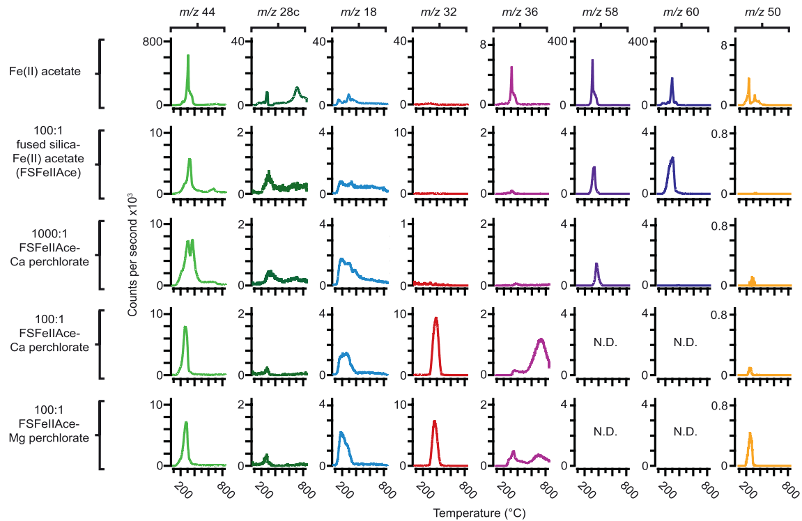
Figure 4. Evolved m/z 44 ( \text{CO}_2 , organic fragments), m/z 28 c (corrected CO, organic fragments), m/z 18 ( \text{H}_2\text{O} , organic fragments), m/z 32 ( \text{O}_2 ), m/z 36 (HCl, organic fragments), m/z 58 (acetone), m/z 60 (acetic acid), and m/z 50 (chloromethane, organic fragments) versus temperature as detected by SAM-like EGA of pure Fe(II) acetate, FSFeIIAce, a 1000:1 FSFeIIAce and Ca perchlorate mixture, a 100:1 FSFeIIAce and Ca perchlorate mixture, and a 100:1 FSFeIIAce and Mg perchlorate mixture. N.D. stands for no detection, which indicates that no signals were detected for m/z 58 and m/z 60 during EGA of the 100:1 perchlorate mixtures. It should be noted that a 1 mg aliquot was used for the pure acetate experiment, 7 mg aliquots for the 100:1 silica and silica-perchlorate mixtures, and a 20 mg aliquot for the 1000:1 mixture. EGA, evolved gas analysis; FSFeIIAce, a 100:1 mixture of fused silica and Fe(II) acetate; SAM, Sample Analysis at Mars.
