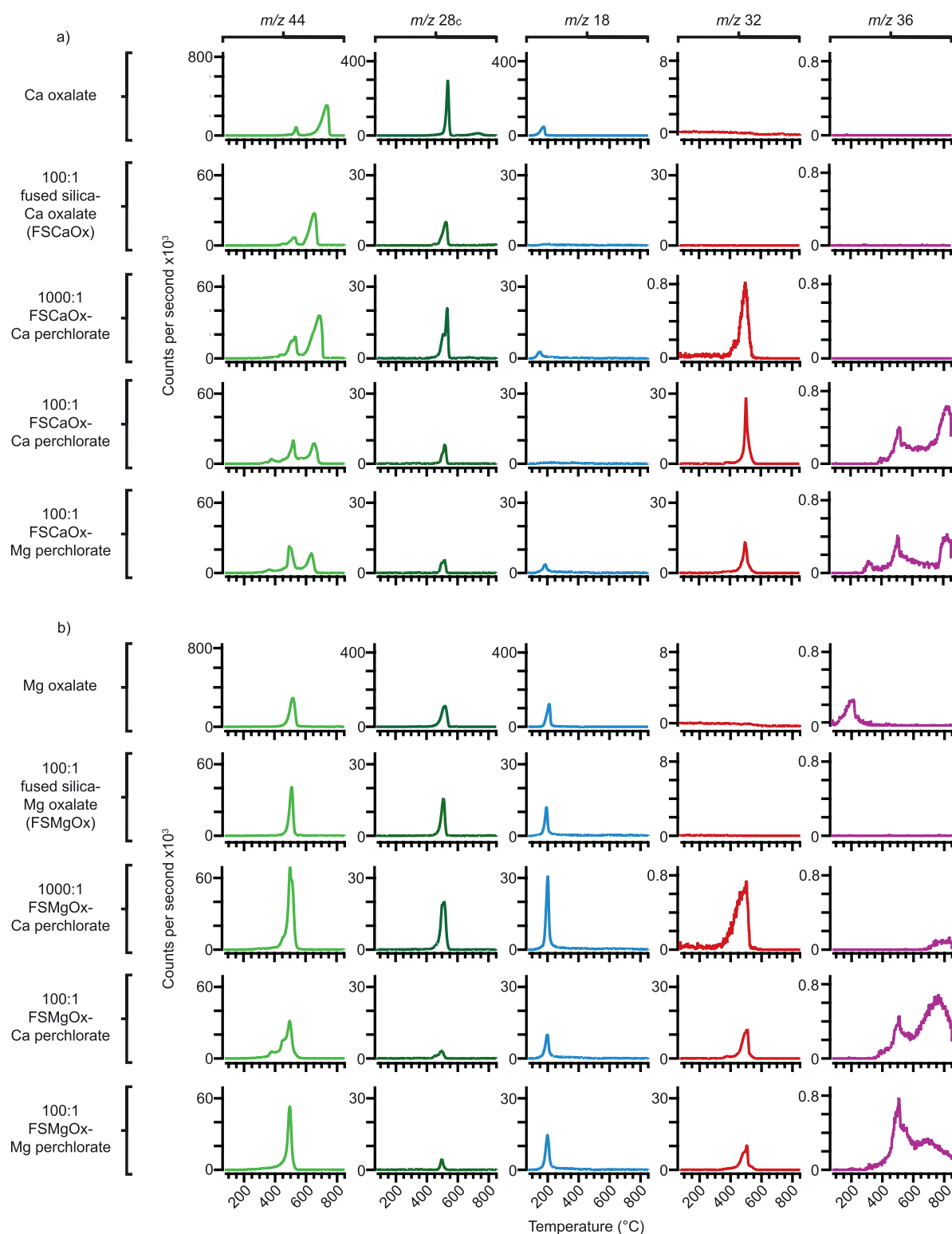
Figure 3. Evolved m/z 44 ( \text{CO}_2 ), m/z 28 c (corrected \text{CO} ), m/z 18 ( \text{H}_2\text{O} ), m/z 32 ( \text{O}_2 ), and m/z 36 ( \text{HCl} ) versus temperature as detected by SAM-like EGA of (a) Ca oxalate and (b) Mg oxalate as pure phases, as FSOx, as 1000:1 FSOx and Ca perchlorate mixtures, as 100:1 FSOx and Ca perchlorate mixtures, and as 100:1 FSOx and Mg perchlorate mixtures. It should be noted that 1 mg aliquots were used for the pure oxalate experiments, 7 mg aliquots for the 100:1 silica and silica-perchlorate mixtures, and 20 mg aliquots for the 1000:1 mixtures. EGA, evolved gas analysis; FSOx, 100:1 mixtures of fused silica and oxalate; SAM, Sample Analysis at Mars.
