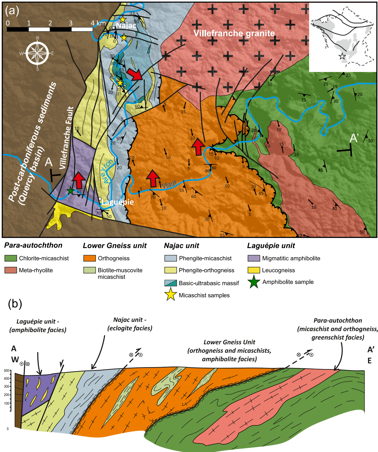
Fig. 1. Geological setting of the Najac and Laguëpie units: (a) geological map modified after Burg et al. (1989a) . The red arrows indicate the kinematics deduced from C'/C/S structures; (b) interpretative W-E cross section with indication of lithology and metamorphic facies for each unit.
