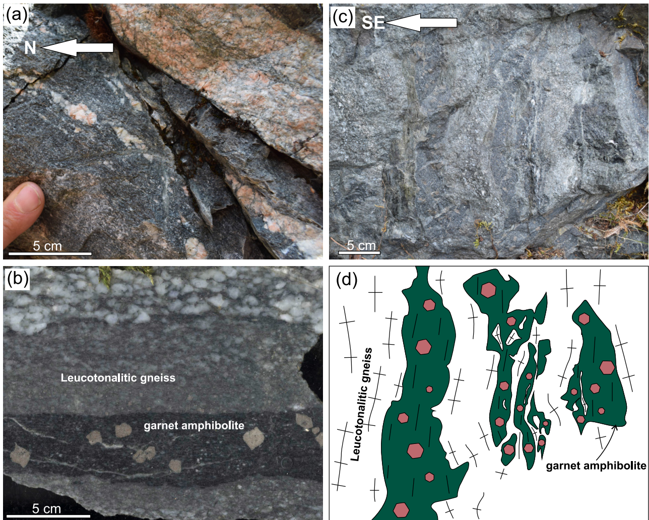
Fig. 2. Main macroscopic features of the Laguéprie unit: (a) field photographs of leucotonalitic lenses into garnet-free amphibolite (AJAH9; 1,9558°E, 44,1485°N); (b) polished section of a garnet amphibolite within a quartz-feldspar-chlorite leucogneiss (AJAH8; 1,9602°E; 44,1468°N); (c) outcrop image of the complex relationship between garnet amphibolite lenses and leucotonalitic veins (1,9602°E; 44,1468°N). Note the crosscutting relationships and the cauliflower-like structure at the leucogneiss/amphibolite contact; (d) sketch of the outcrop image shown in (c).
