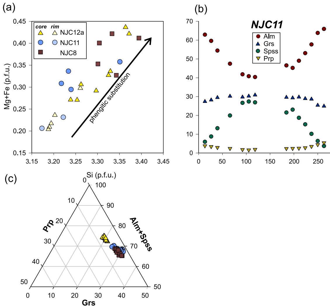
Fig. 5. Minerals composition in the micaschists from the Najac unit: (a) Si versus Fe+Mg diagram for white micas showing the phengitic substitution; (b) garnet zoning profile in NJC11; (c) garnet composition for three representative samples (NJC8, NJC11 and NJC12a).
