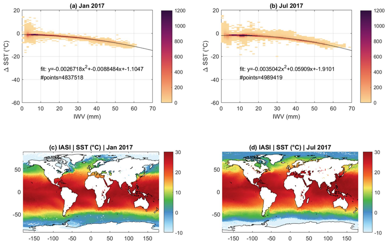
Figure 3. (a) SST bias fit as a function of IWS for January 2017; (b) Same as (a) but for July 2017; (c) Corrected IASI-derived monthly mean SST for January 2017; (d) Same as (c) but for July 2017.
