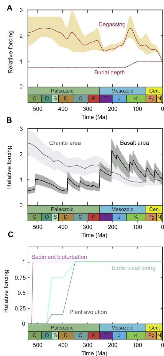
Fig. 3. Nondimensional forcings. A. Tectonic forcing controlling input rate of \text{CO}_2 . B. Land area forcings affecting the strontium isotope composition of silicate weathering fluxes. C. Biological forcings affecting carbon burial and weathering. All are based on the COPSE model.
