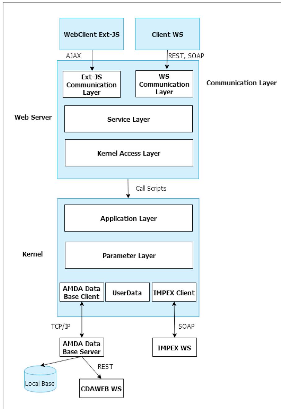
Fig. 3. General architecture of AMDA (see text for details).
