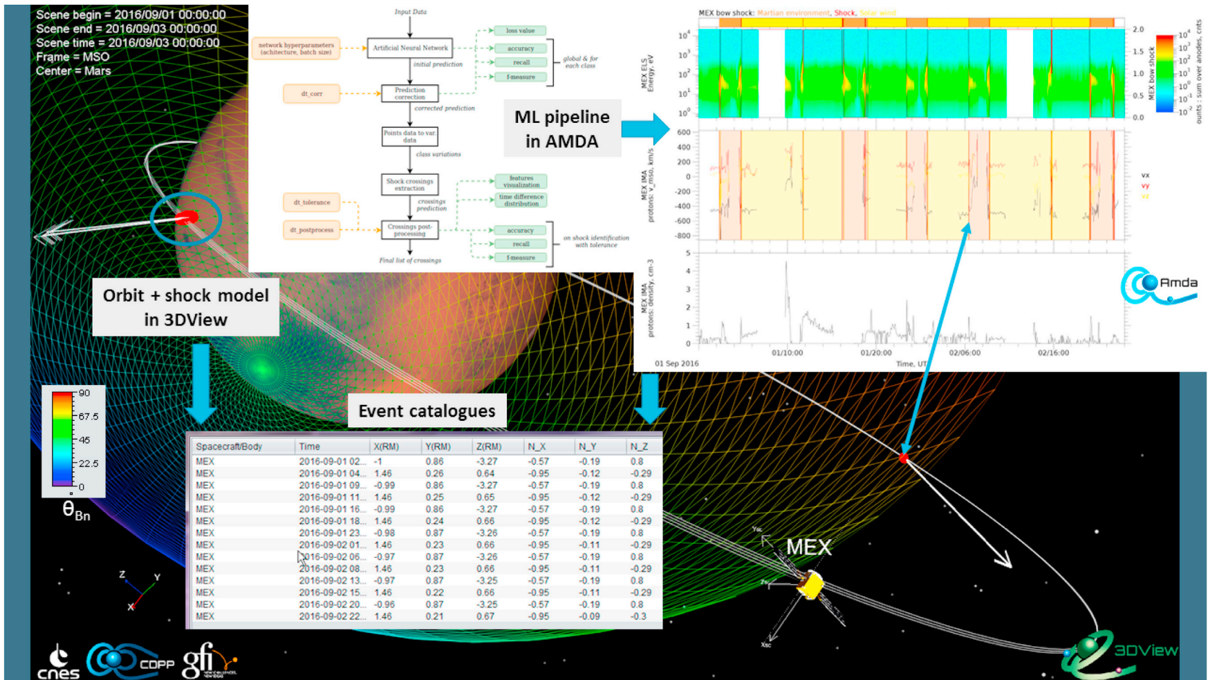
Fig. 12. Detection of plasma regions around Mars from Mars Express data: a supervised machine learning algorithm (top left) has been trained to detect solar wind/bow shock/planetary environment. The ‘predicted’ regions form a catalogue (bottom left) are shown to the AMDA user both as a colour chart above the data and with coloured intervals (top right) as an help to understand the observational context. The underlying illustration is a 3DView scene which makes use of the same catalogue for 3D display of the shock crossings and normals by the MEX spacecraft. The wired surface is a shock model coloured by the values of the shock angle ( \theta_{Bn} ).
