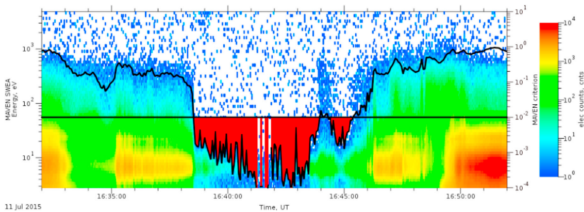
Fig. 10. Electron depletions (red regions between black lines) seen by MAVEN and detected in AMDA from the criterion proposed in Steckiewicz et al. (2017) (see the text for details). The spectrogram is from the SWEA instrument (electron counts).
