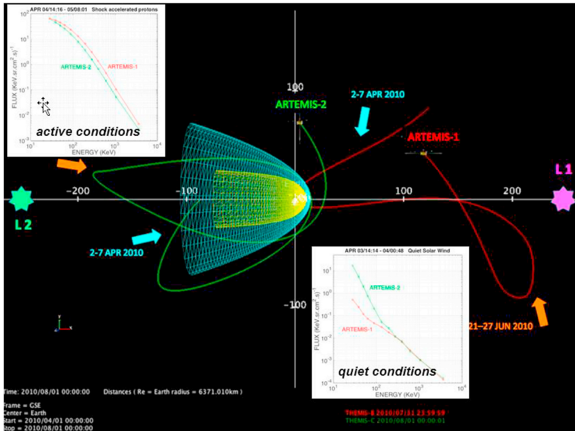
Fig. 11. Comparison of the spectra obtained by ARTEMIS-1 in the solar wind and ARTEMIS-2 in the distant tail or magnetosheath during active (upper left) and quiet (bottom right) solar conditions. Because the particle environment at L2 is likely to be worse in terms of ATHENA background, the AMDA-based analysis showed there is no benefit to placing ATHENA at L2 versus L1 (see text for details). The background image is a 3DView XZ GSE view of the magnetosphere between L1 and L2 (magnetopause and shock models are seen in yellow and blue respectively) with trajectories of both ARTEMIS spacecraft.
