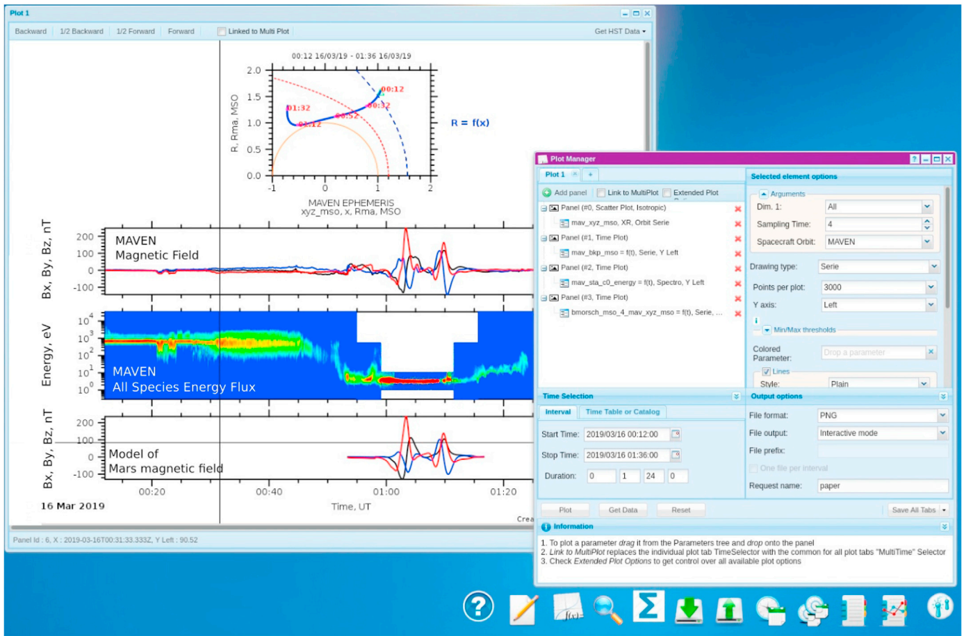
Fig. 1. A generic AMDA screen. The plot window shows the MAVEN orbit about Mars, MAVEN magnetic field data, MAVEN Energy-Time spectrogram of the ion energy flux, and the Morschhauser et al. (2014) model of the martian crustal magnetic field calculated along the MAVEN orbit. The right hand side window shows the “plot request” panel set up for this plot. Icons at the bottom right are short cuts to the different analysis activities described in the paper.
