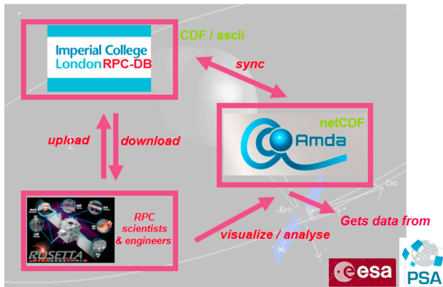
Fig. 15. Architecture of the Imperial College-AMDA collaboration for Rosetta Plasma distribution to the Consortium during the operational phase. In the post-operational phase the data were obtained from PSA when available (bottom right).
