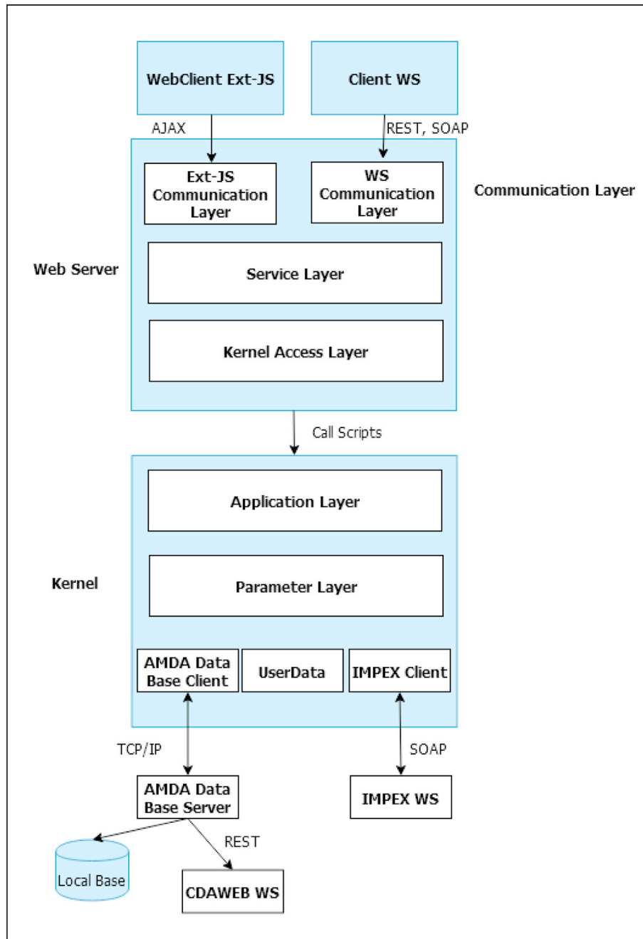
Fig. 3. General architecture of AMDA (see text for details).
