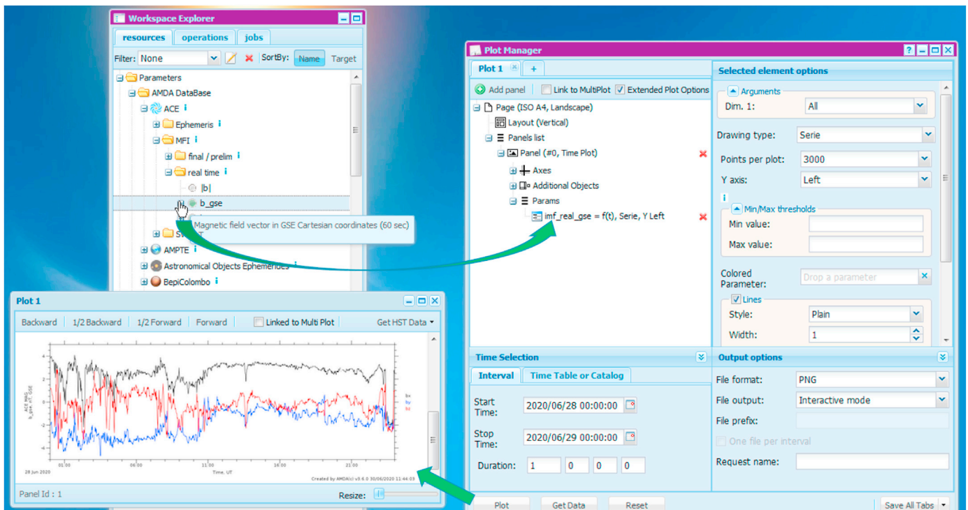
Fig. 4. Plotting a parameter in AMDA is realized by drag and dropping a parameter from the Workspace Explorer to the Plot Manager (upper green arrow). The plot interface shows the panel composer (upper left), the time selection (bottom left), the plot customization options (upper right) and output selection (bottom right). Activating the “Plot” button produces a figure (second green arrow). The example shows “Real Time” ACE magnetic field vector in GSE (with internal parameter ID = ‘imf_real_gse’) selected for 1 day. A tooltip is shown when the mouse is over a parameter with the full parameter name, resolution and unit.
