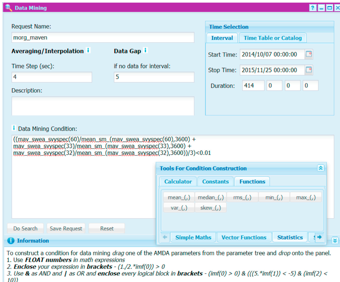
Fig. 6. The conditional search interface. The windows are filled with parameters extracted from the MAVEN use case detailed in Section 6.1.1.
