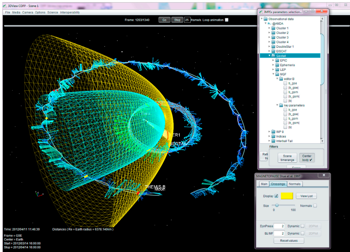
Fig. 7. Themis-B and Geotail magnetic field vectors obtained from AMDA and plotted in a magnetospheric scene in 3DView (the amplitude of the field is coded in both length and color). The main window shows about a month of data (mid-March to mid-April 2012): the trajectory of Themis-B orbiting around the moon, and several orbits of Cluster 1 and Geotail; also shown are the bowshock (Fairfield, 1971) and magnetopause (Shue et al., 1997) modeled surfaces in yellow and blue respectively. Red and yellow bullets are the crossing locations of these two boundaries by orbiting objects, spacecraft and the moon. The inset windows on the right shows the 3DView access to AMDA (top) and the control panel for the magnetopause model bottom (bottom). Other control panels are not shown.
