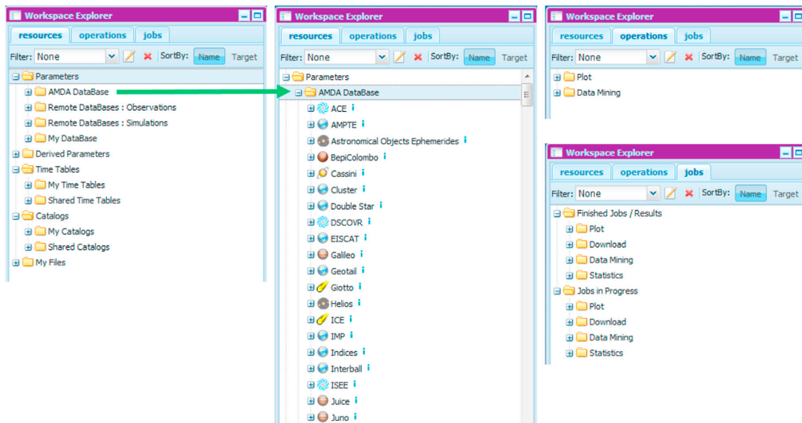
Fig. 2. The Workspace Explorer with the three tabs “resources” (left), “operations” (top right) and “jobs” (bottom right). The middle image is a view of AMDA database resources (by alphabetical order, from A to J only on this view) and shows directories for spacecraft missions, radar, indices, and ephemeris.
