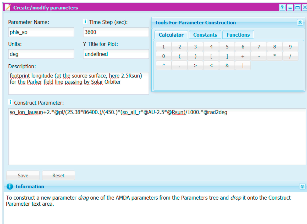
Fig. 5. The parameter editor interface. The example shows how to construct the magnetic footprint longitude \varphi_s of the Solar Orbiter spacecraft as given by Equation (1) (see Section 6.1.5); the time resolution is 1 h and the unit ‘deg’ for degree. The parameter IDs which appear in the “Construct Parameter” edit window have been obtained by drag&dropping of the corresponding (explicit) parameters from the Workspace Explorer (similar to the drag&drop action for the Plot, see Fig. 4). The variables starting with “@” are built-in constants found in the “Constants” tab (common physical constants, planetary radii, ...).
