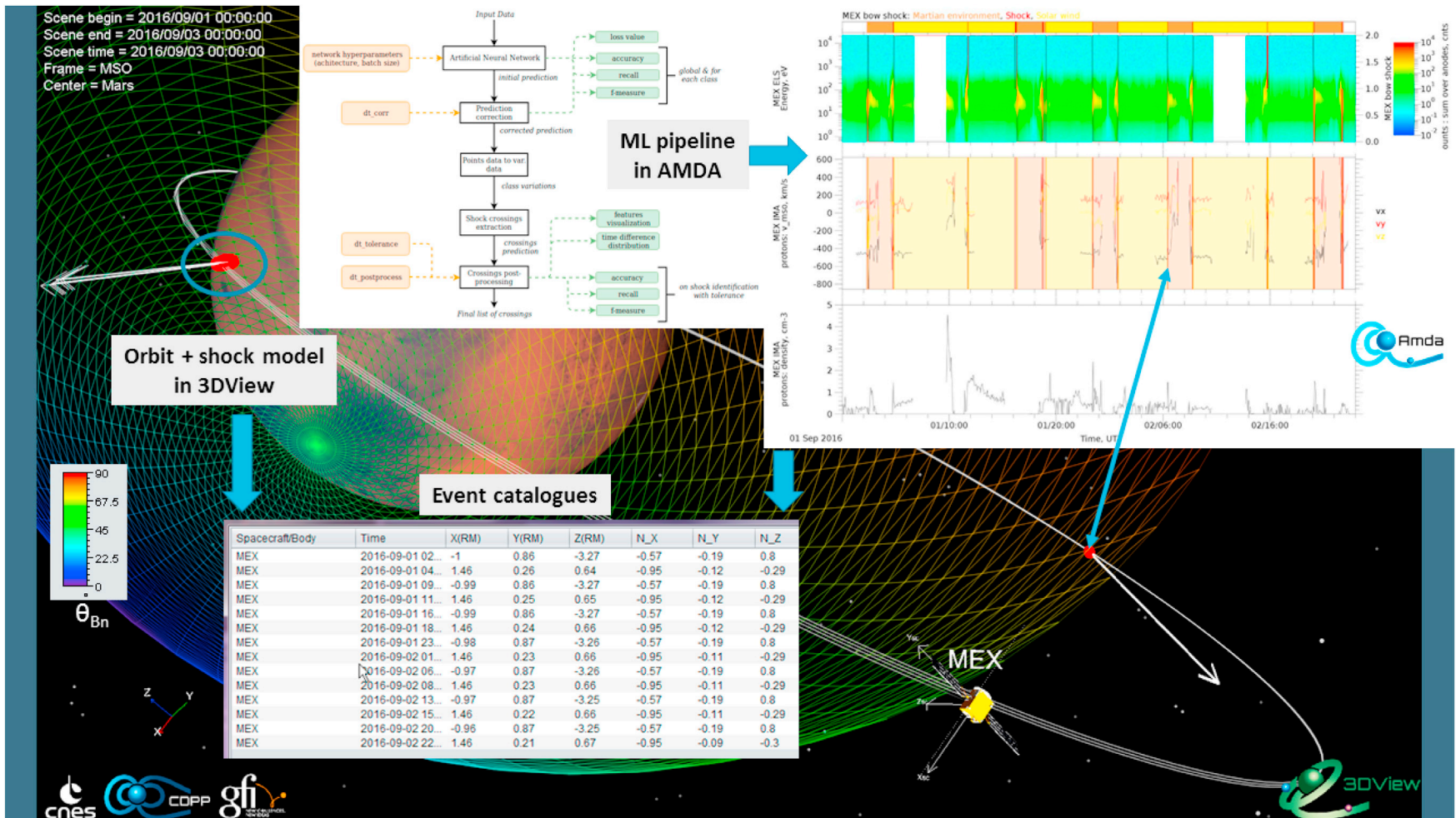
Fig. 12. Detection of plasma regions around Mars from Mars Express data: a supervised machine learning algorithm (top left) has been trained to detect solar wind/bow shock/planetary environment. The ‘predicted’ regions form a catalogue (bottom left) are shown to the AMDA user both as a colour chart above the data and with coloured intervals (top right) as an help to understand the observational context. The underlying illustration is a 3DView scene which makes use of the same catalogue for 3D display of the shock crossings and normals by the MEX spacecraft. The wired surface is a shock model coloured by the values of the shock angle ( \theta_{Bn} ).
