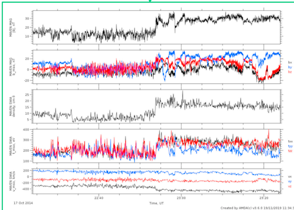
Fig. 8. Study of the 14 October 2014 (Sun time) Interplanetary Coronal Mass Ejection (ICME) with the Propagation Tool and AMDA; a full report is available in Witasse et al. (2017). The above plot shows the Propagation Tool interface in which the ICME parameters have been filled to compute the propagation from the Sun to MAVEN with a predicted arrival on 2014-10-17T22:54:32. By clicking on “CDPP interface” (1) the small inset window enables users to choose which in-situ parameters are plotted in AMDA. Here MAVEN magnetic field and plasma moments are chosen for 2 h centered on the arrival time. Clicking on “AMDA plot” generates the bottom plot (2) in the browser: within a few tens of second from the centre time (predicted by the Propagation Tool) the jumps in all parameters are typical of the ICME passage.
