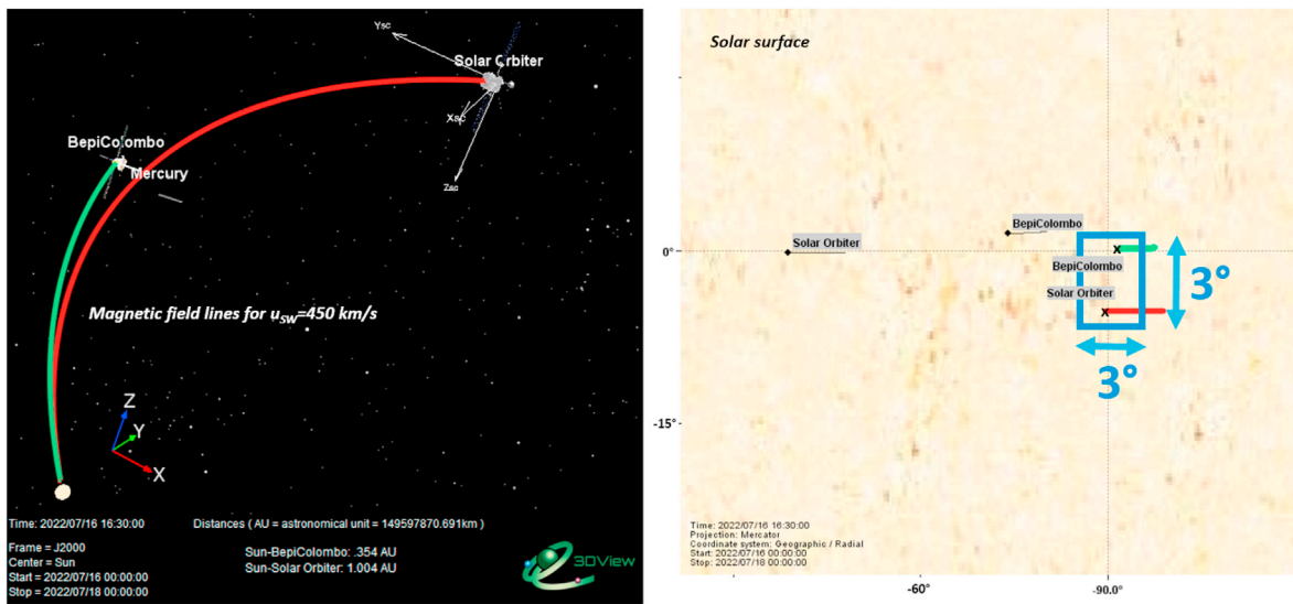
Fig. 14. 3DView illustration of the solar magnetic connectivity of BepiColombo (green) and Solar Orbiter (red) for the third interval of Table 3 when the 2 spacecraft have magnetic footprints (crosses on the right-hand side at the solar source surface) co-located in a 3^\circ \times 3^\circ longitude/latitude box. The lines are displayed for u_{SW} = 450 km/s. The diamond symbols are the radial footprints (sub-spacecraft points).
