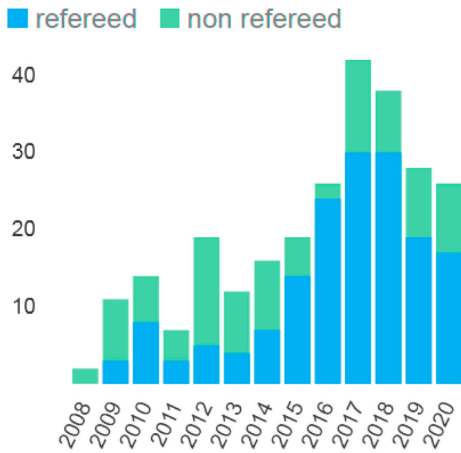
Fig. 16. Distribution of papers acknowledging AMDA over the period 2008–2020 obtained from the SAO/NASA Astrophysics Data System (as of 07/12/2020).
