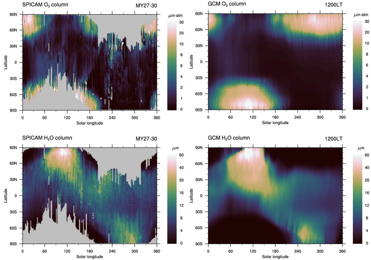
Figure 2. Climatologies of SPICAM ozone and water vapor as a function of L_s and latitude, compared to the LMD GCM nominal simulation. Left: SPICAM O_3 (top) and H_2O (bottom) column, averaged over Mars years 27 to 30. The columns are zonally averaged and binned by 2^\circ in L_s and 2^\circ in latitude. Right: LMD GCM nominal simulation of O_3 (top) and H_2O (bottom) calculated at 1200 local time. Units are \mu\text{m-atm} for ozone and \text{pr-}\mu\text{m} for water vapor.
