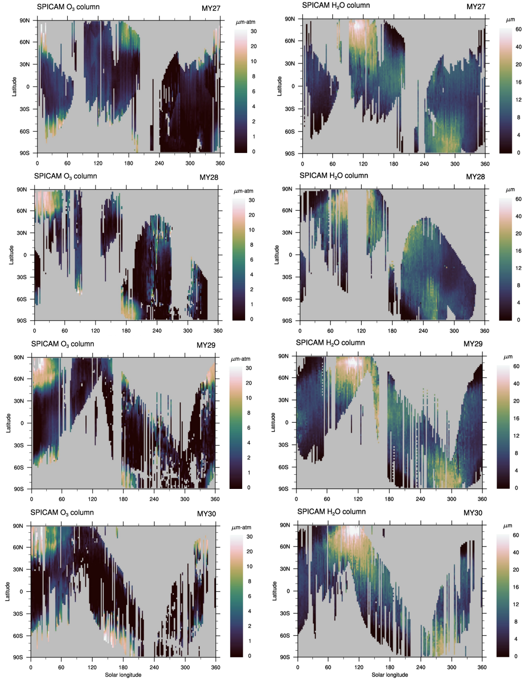
Figure 1. Overview of the SPICAM ozone (left) and water vapor (right) column abundance as a function of season, latitude, and Mars year. The columns are zonally averaged and binned by 2^\circ in L_s and 2^\circ in latitude. Units are micron-atmosphere ( \mu\text{m-atm} ) for ozone and precipitable micron ( \text{pr-}\mu\text{m} ) for water vapor.
