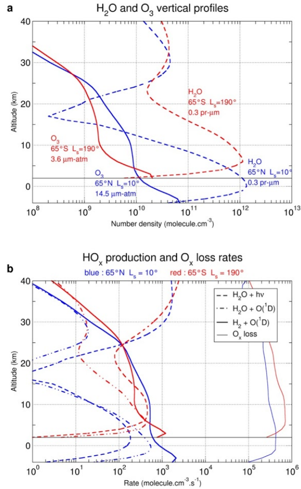
Figure 4. Examples of profiles of O 3 , H 2 O, and production/loss rates calculated by the LMD GCM at high latitudes in early spring. Altitude is relative to the Mars areoid and local time is 1200. (a) O 3 and H 2 O number densities at 65°N (L s = 10°) and 65°S (L s = 190°). (b) HO x production rate for the most important reactions and O x loss rate at 65°N (L s = 10°) and 65°S (L s = 190°).
