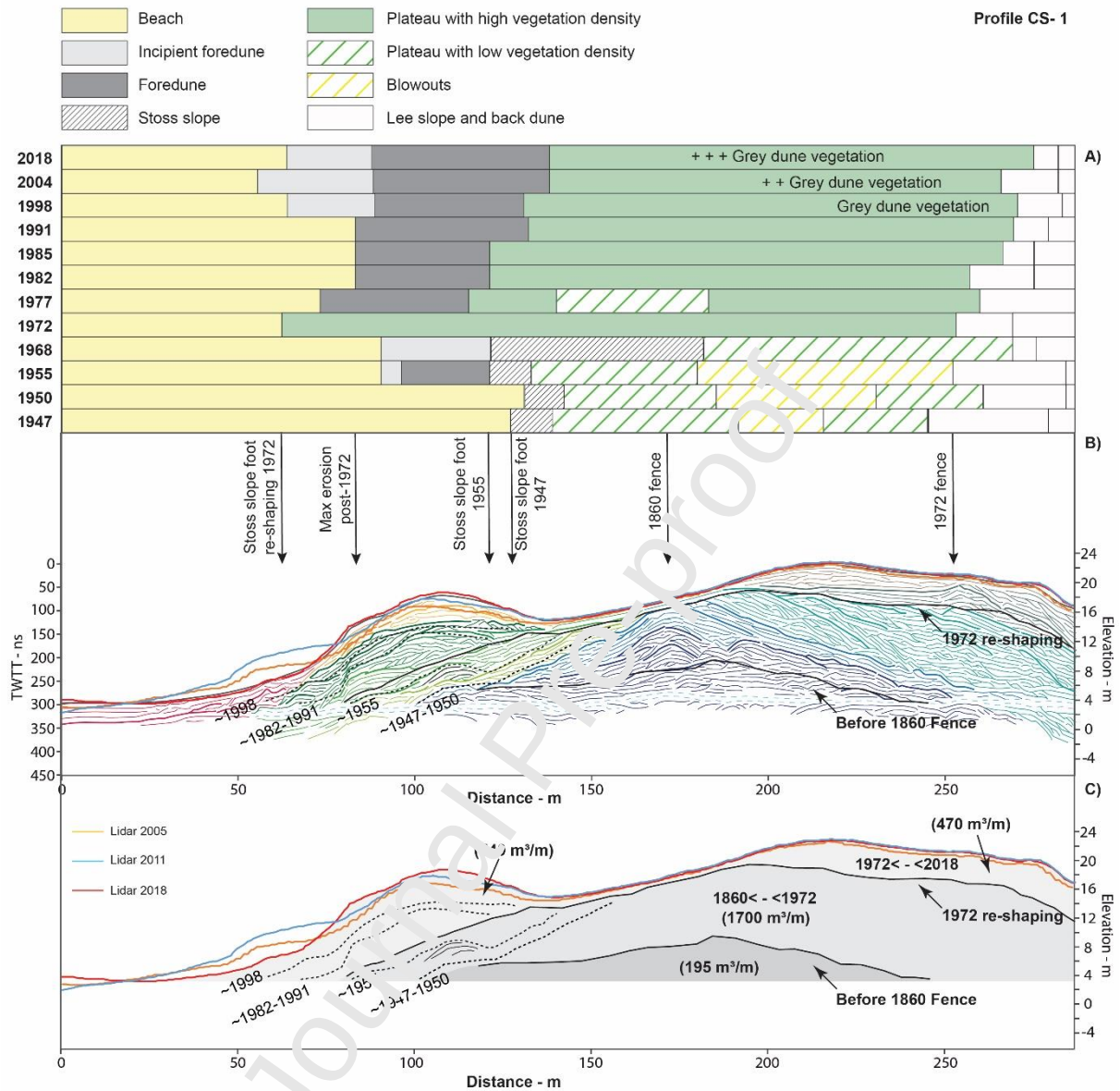
Fig.10: CS-1 profile with (a) geomorphology and interpretation of dune morphology between 1947 and 2018; (b) reflection-traced version of radar units and interpretation of several paleotopographic profiles; (c) estimation of dune volume during several periods (before 1860, between 1860 and 1972, post 1972). Elevation in meters above mean sea-level (amsl).
