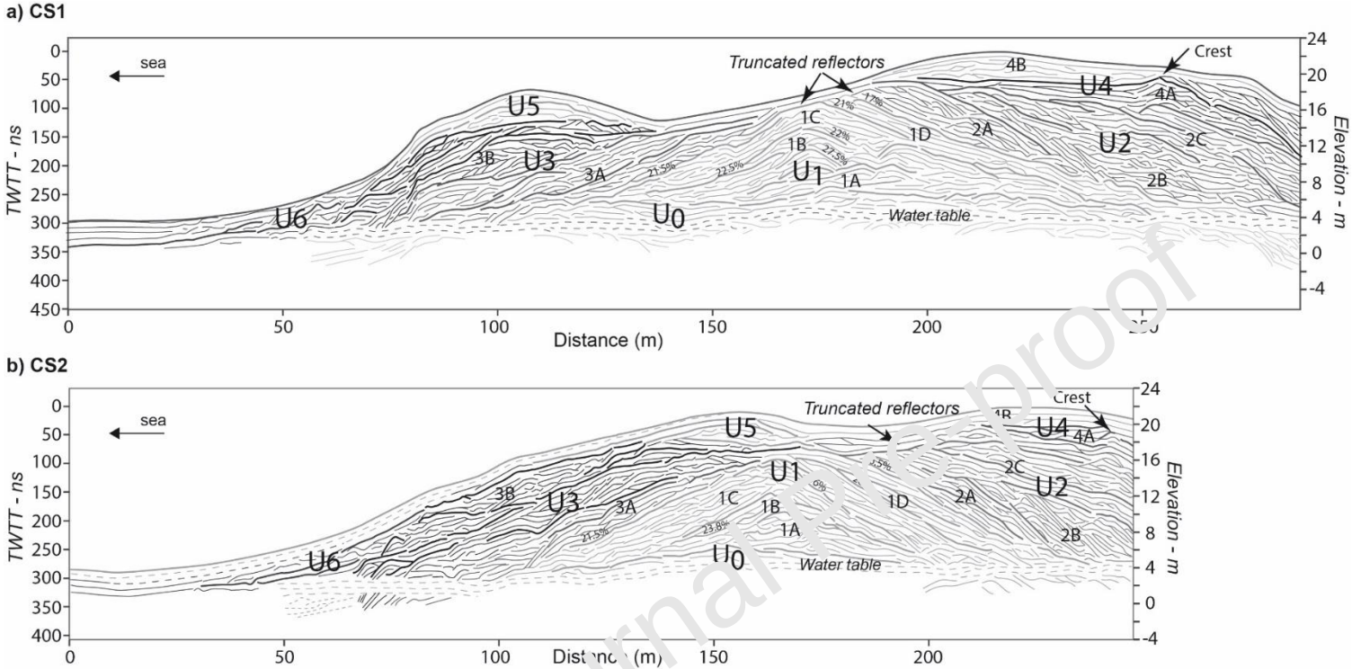
Fig.9: Reflection-traced version of radar units defining the internal architecture of the dune acquired with 100 MHz frequency antennae. (a) CS-1 profile and (b) CS-2 profile. GPR data are given in nanosecond (ns) two-way travel time (TWTT) and elevations are with reference to mean sea-level (amsl).
