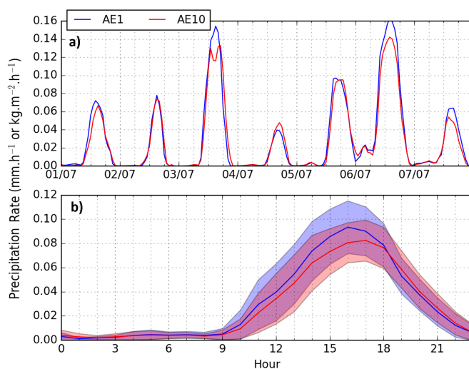
Figure 10. Time series (top) and diurnal cycles (bottom) of modeled hourly precipitation rate ( \text{kg}\cdot\text{m}^{-2} ) for the two experiments, AE1 (blue) and AE10 (red), averaged over an inland area extending from 7^{\circ}\text{N} to 9^{\circ}\text{N} , and from 1^{\circ}\text{E} to 4^{\circ}\text{E} for the period 1–7 July 2016. (a) The vertical dashed lines indicate periods of 6 hours starting at 00:00 UTC. (b) Means of each hour for the period 1–7 July 2016 are presented by lines, and the upper and lower shading limits correspond to the hourly standard deviation.
