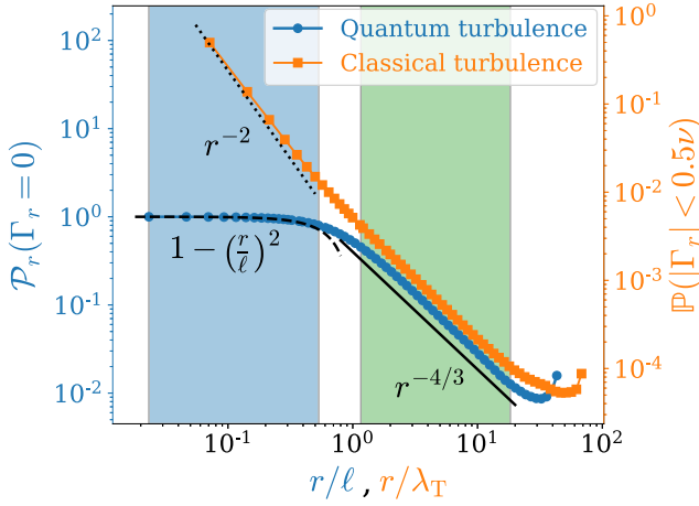
FIG. 6. Probability of having zero circulation in gGP simulations (blue line) and of having a weak circulation in Navier-Stokes simulations (orange line). The dashed lines show their respective predictions at large and small scales.
