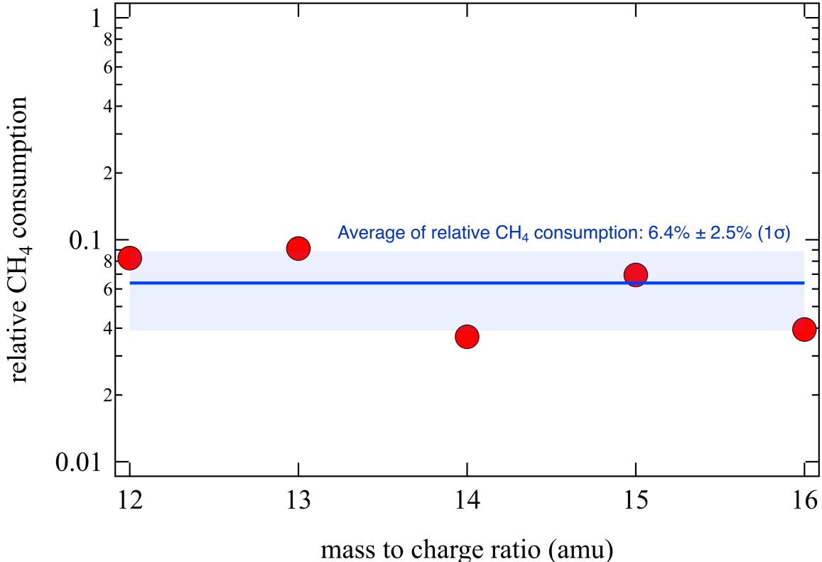
Figure 1: Relative methane consumption ( ((CH_4)_0 - (CH_4)_t) / (CH_4)_0 ) during one hour of EUV irradiation of a N_2/CH_4 mixture (90/10%) at 0.1 mbar. Each mass related to methane was used to obtain a value of the relative methane consumption (red dots). The blue line is the average of the red dots and the blue area displays the standard deviation.
