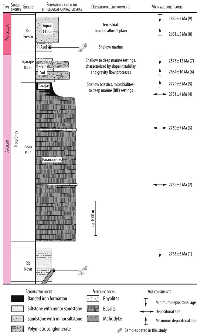
Fig. 2. Main sedimentary units of the Carajás Basin. Stratigraphic column adapted after Araújo Filho et al. (2020); Araujo and Nogueira (2019); Klein and Ladeira (2002); Machado et al. (1991); Trendall et al. (1998). References for age constraints are given in Table 1.
