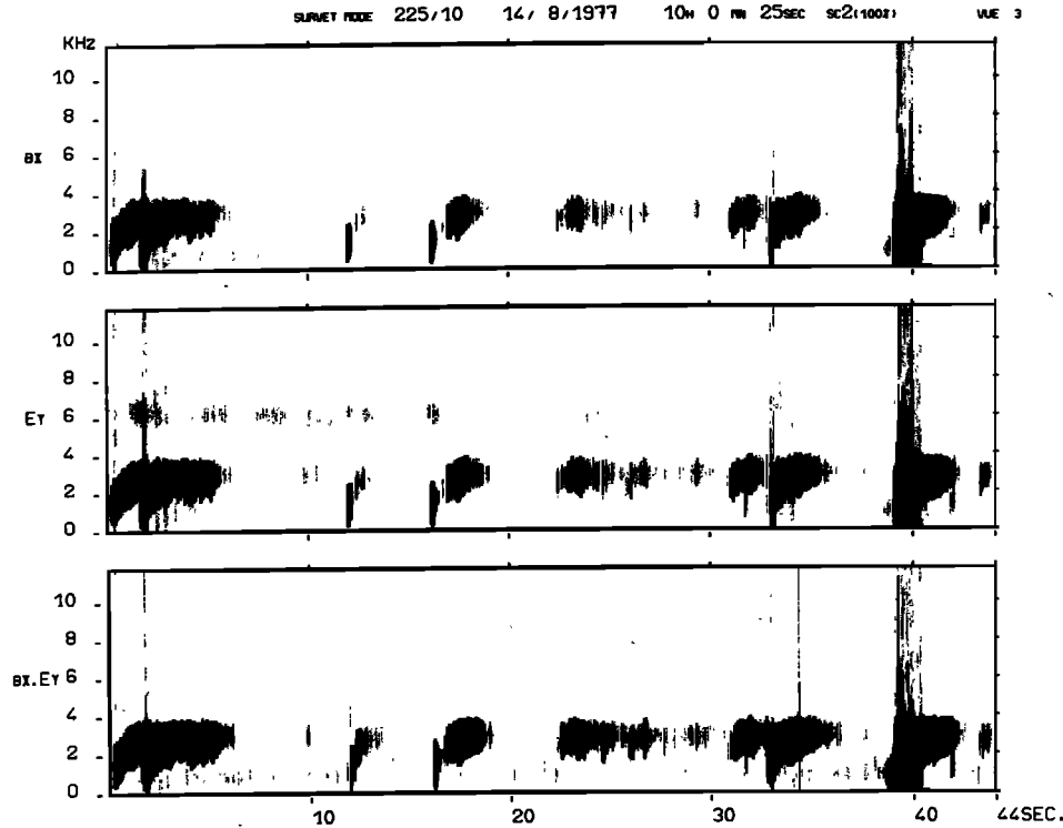
Fig. 7. Auto and cross-spectra on b_x and E_y for the VLF emission event on August 14, 1977, around 1000 UT. The orbit parameters are: LT = 1148, Dist = 5.95, L = 6.01, LAT = 5^{\circ}7' , lat = 0^{\circ}80' , long = 25^{\circ}10' , \alpha = 12^{\circ}06' . The estimated plasma parameters are \Omega_e = 4.42 kHz, \Pi_e = 23.7 kHz.
