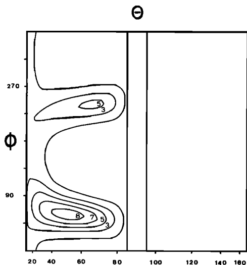
Fig. 10. Maximum entropy solution for the hiss event on June 20, 1977 (see Figures 3 and 4), for N = 36 and M = 9 . The quality parameters are Q = 0.43 , P_r = 2.33 .
