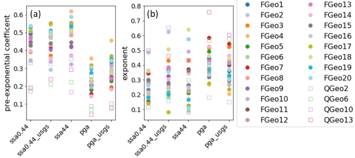
Figure 5. (a) pre-exponential coefficient and (b) exponent of eqn(11) for all Finney pack geometries (filled circle), and the subset of quartz sand pack geometries simulated (open square) for different precipitation kinetic setups.
