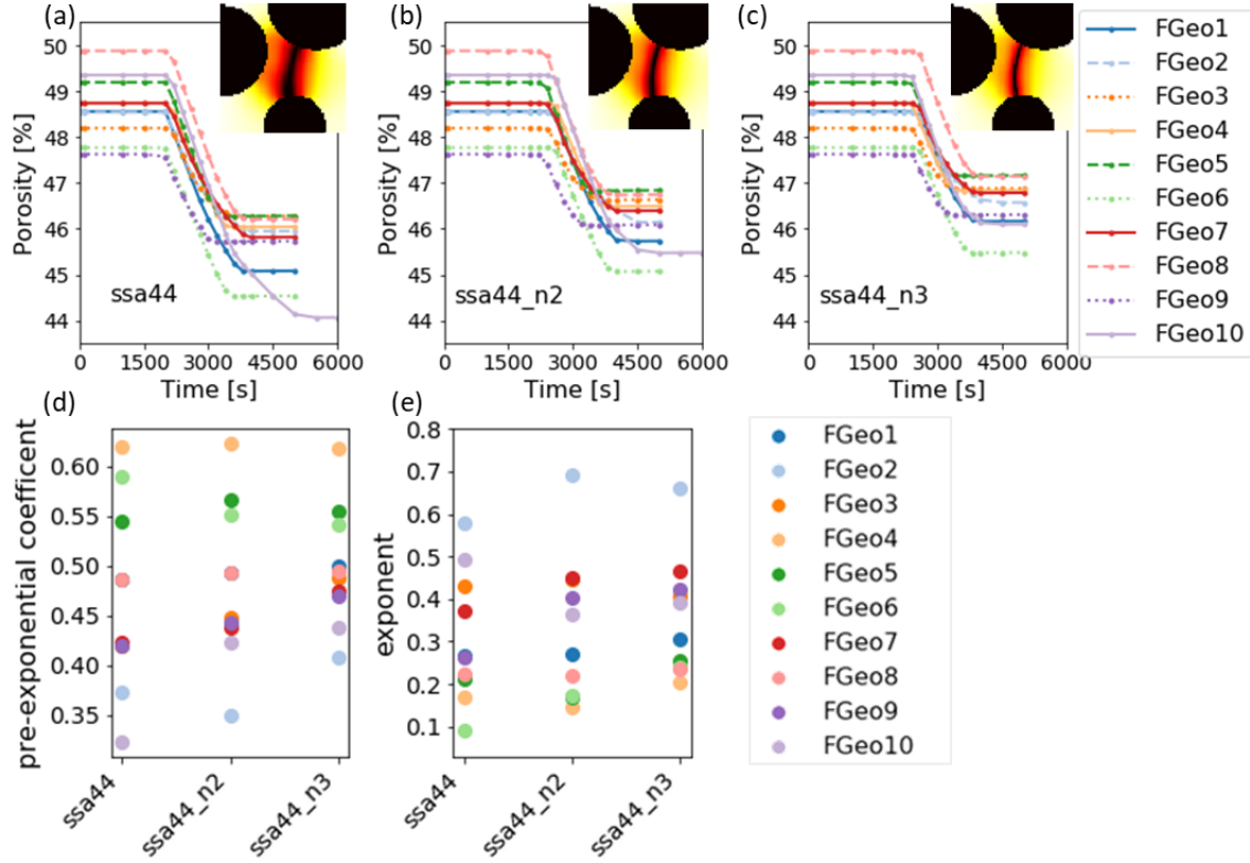
Figure 6. Comparison of the porosity evolution of ten Finney pack geometries using the default linear grid-cell level tortuosity model (a), the nonlinear tortuosity model with exponent of 2 (b) and 3 (c), and the pre-exponential coefficient (d) and exponent (e) of the \Phi - D_{eff} relationship of the three cases.
