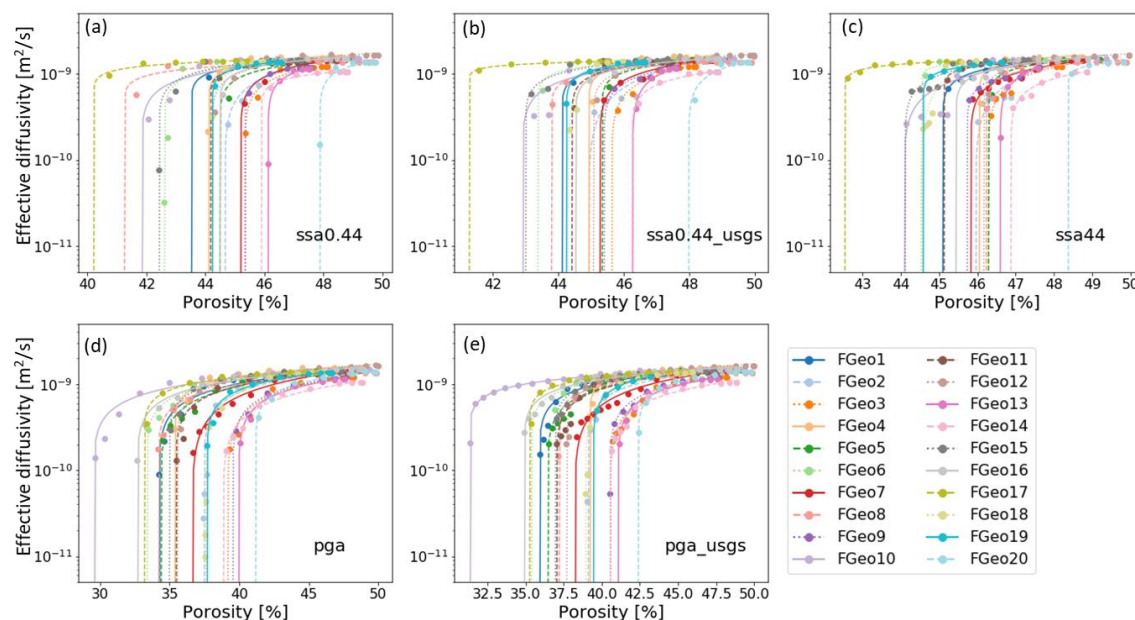
Figure 4. Effective diffusivity in relation to the porosity from the tracer simulations and the fitting line using eqn(11) for the five precipitation kinetic setups of all the Finney pack geometries (FGeo1-20). The goodness-of-fitting R2 parameter is 0.97 on average, and larger than 0.91 for all 100 cases except for two.
