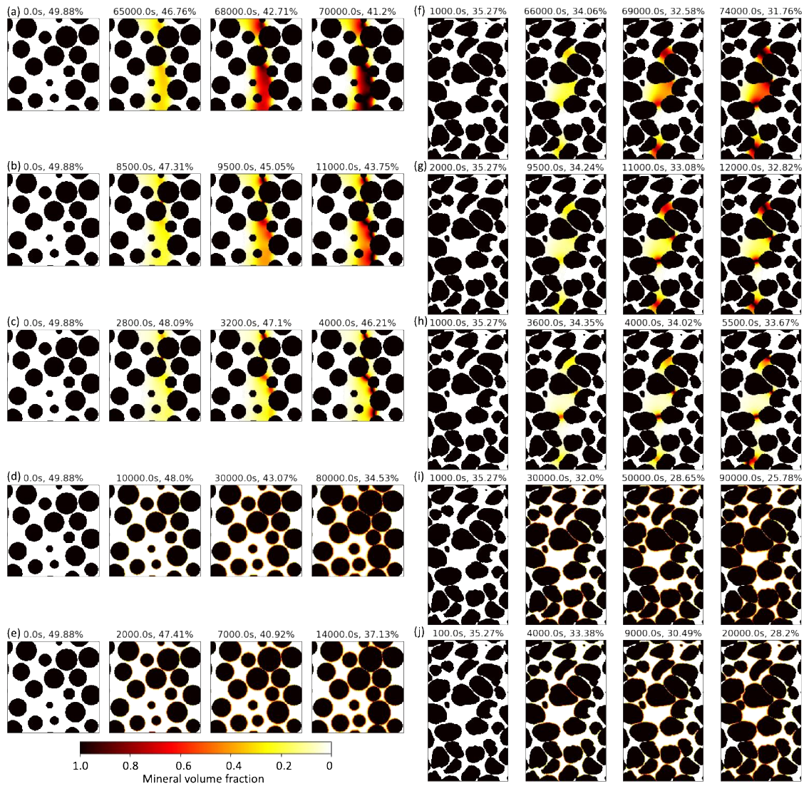
Figure 2. Snapshots of pore geometry evolution for a Finney pack geometry (a-e) and a quartz sand pack geometry (f-j) for different precipitation setups: (a)(f) – ssa0.44, (b)(g) - ssa0.44_usgs, (c)(h) – ssa44, (d)(i) – pga, (e)(j) – pga_usgs. Note: due to the difference in reaction rate and geometry, each case reached the clogging point at different time steps and the snapshots shown are thus at different times.
