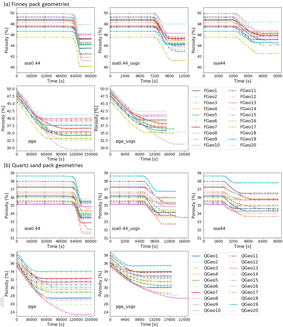
Figure 3. Domain porosity ( \Phi ) evolution for (a) twenty Finney pack geometries (FGeo1-20) and (b) twenty quartz sand pack geometries (QGeo1-20) with different precipitation setups. Note: some cases had longer simulations as they required longer to reach the clogging time point than other cases.
