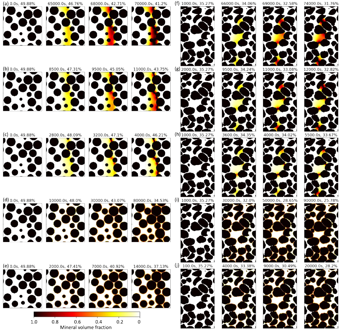
Figure 2. Snapshots of pore geometry evolution for a Finney pack geometry (a-e) and a quartz sand pack geometry (f-j) for different precipitation setups: (a)(f) – ssa0.44, (b)(g) – ssa0.44_usgs, (c)(h) – ssa44, (d)(i) – pga, (e)(j) – pga_usgs. Note: due to the difference in reaction rate and geometry, each case reached the clogging point at different time steps and the snapshots shown are thus at different times.
