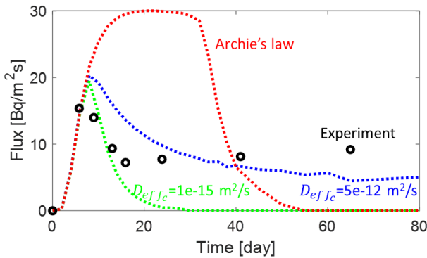
Figure 7. Tracer flux at the outlet. The experimental observations are shown in the open black circles, in comparison with simulations results using the traditional form of Archie's law (red dotted line), and using the revised relationship with D_{effc} = 1 \times 10^{-15} \text{ m}^2/\text{s} (green dotted line) and D_{effc} = 5 \times 10^{-12} \text{ m}^2/\text{s} (blue dotted line).
