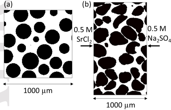
Figure 1. Illustration of the 2D domains of (a) the Finney pack geometry and (b) the quartz sand pack geometry, and of the fluid chemistry boundary conditions used in the simulations.
