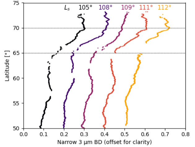
Figure 7: Profiles of the latitudinal evolution of the narrow 3 \mu\text{m} BD (offset for clarity) from several L_s observations of the Phoenix landing site region at different L_s (orbits 0979, 1001, 1012, 1023 & 1034). Each point is averaged in longitude between 235°E and 240°E (image lines), considering only the pixels with a surface reflectance at 2.26 \mu\text{m} between 0.3 and 0.35 to avoid albedo effects in the latitudinal trends of the band depth estimators. Profiles are then smoothed using a moving average.
