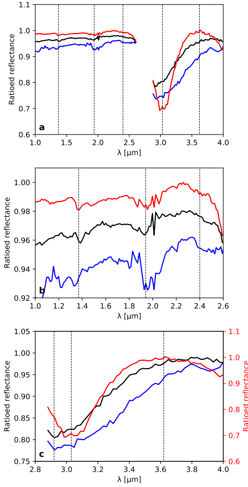
Figure 6: (a) A typical averaged spectral ratio corresponding to the 3 \mu\text{m} northern ring identified in this study (red) is compared to a ratio obtained outside the ring between 50°N and 60°N (black), and to a ratio from southern bright terrains between 62°S and 74°S (blue). Black dotted lines correspond to wavelengths of 1.37, 1.94, 2.4, 3.03, and 3.62 \mu\text{m} . The red spectrum is the average of 4 ratioed spectra taken along the narrow 3 \mu\text{m} northern ring (longitudes \sim 15^\circ\text{E} / 135^\circ\text{E} / 240^\circ\text{E} / 265^\circ\text{E} ). Each one is the ratio of the average of 200 spectra in a bright region at latitude \sim 70^\circ\text{N} over a similar region in albedo at the same longitude and at latitude \sim 63^\circ\text{N} , then normalized with the reflectance at 2.26 \mu\text{m} before averaging ratios from different longitudes. The black spectrum is the average of 3 spectra acquired at different longitudes ( \sim 15^\circ\text{E} / 240^\circ\text{E} / 265^\circ\text{E} ). Each one is the ratio of 200 pixels from a bright region at \sim 60^\circ\text{N} over a region with a similar albedo at the same longitude at \sim 50^\circ\text{N} . The blue spectrum is the average of 2 spectra acquired at different longitudes ( \sim 140^\circ\text{E} / 205^\circ\text{E} ). Each one is the ratio of 200 pixels from a bright region at \sim 74^\circ\text{N} over a region with a similar albedo at the same longitude at \sim 62^\circ\text{N} . (b) & (c) Zooms on the signatures of the C and L channels respectively. On panels (a) & (b) the blue and black spectra have been offset for clarity. On the panel (c) the y-scale of the red spectrum has been adjusted independently for clarity.
