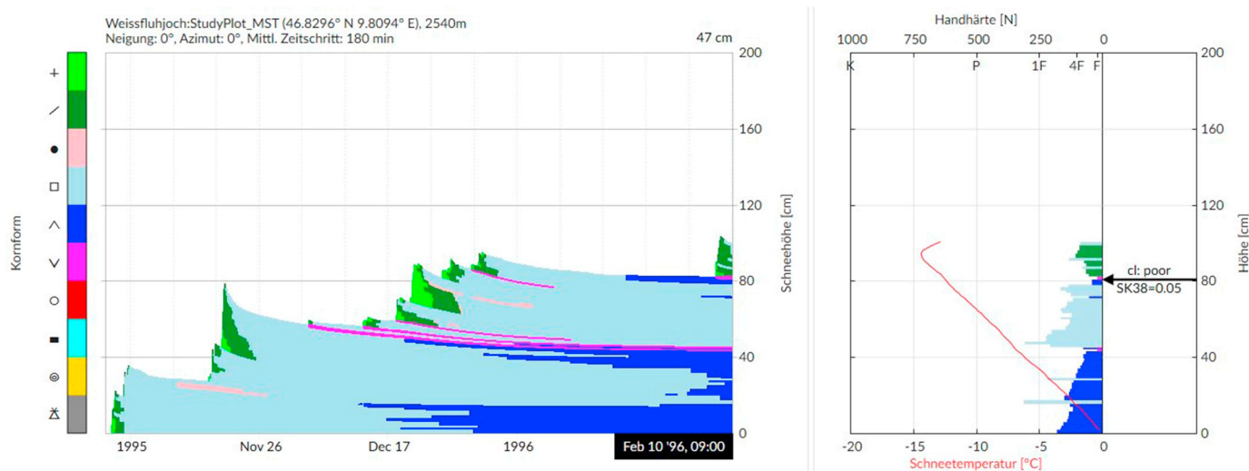
Fig. 4. Visualization of the time series of the snow type vertical profile at the Weissfluhjoch field site near Davos, Switzerland during the snow season 1995–1996. On the right hand side, close-up on the vertical profile at a selected date, showing the layering of snow type and hand hardness.
