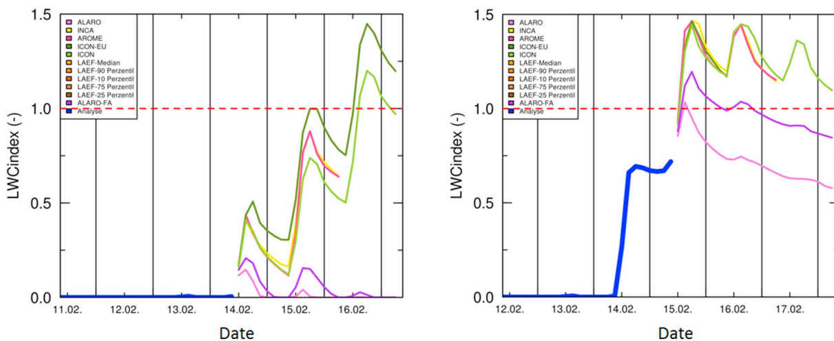
Fig. 9. LWC_{index} ensemble forecasts for south-facing slopes in the Eastern Alps (Hochschwab, Sonnshienalm, 1520 m). Left: 14 February 2017, 11:00 Mitteleuropäische Zeit (MEZ); Right: 15 February 2017, 11 MEZ. Blue: Nowcast; Coloured: Forecasts based on different NWP models. The lines show the LWC_{index} from the retrospective SNOWPACK simulation for a south-facing slope with a slope angle of 38 degrees. The blue line represents the nowcast (i.e. SNOWPACK is driven by meteorological observations) and the coloured lines represent the forecasts from different NWP models (i.e. SNOWPACK is driven by an ensemble of NWP models). (For interpretation of the references to colour in this figure legend, the reader is referred to the web version of this article.)
