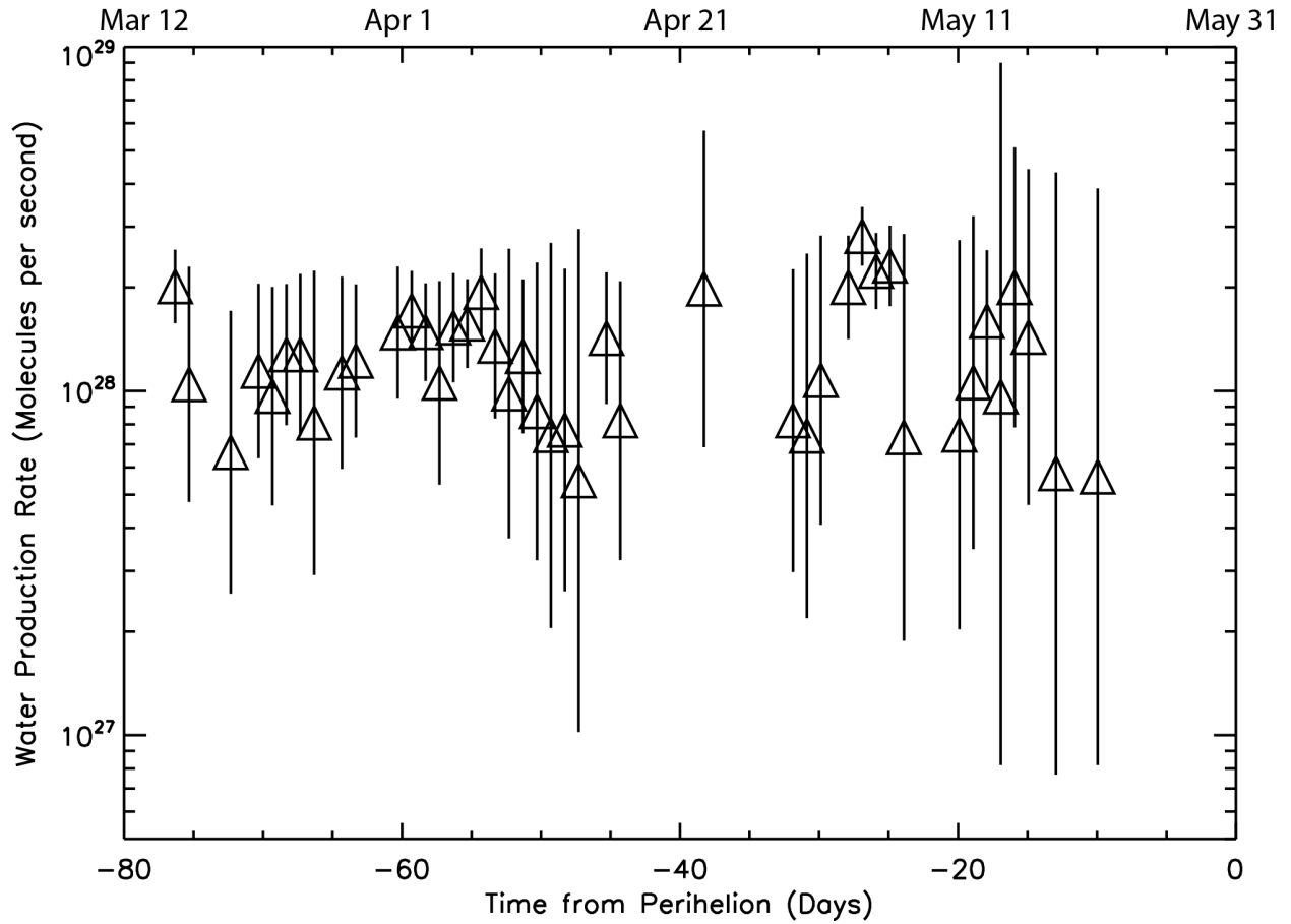
Figure 7. Water production rate in comet C/2019 Y4 (ATLAS) as a function of time from perihelion and UT date 2020. The points give the water production rate in s^{-1} from single images. The error bars give the 1-\sigma formal random fitting errors for each value. There is a \sim 30\% uncertainty from the model parameters and calibration.
