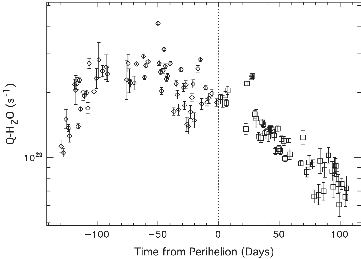
Figure 2. Water production rate in comet C/2009 P1 (Garradd) as a function of time from perihelion. Figure from Combi et al. (2013).
