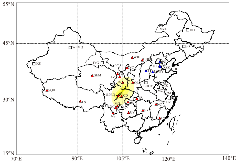
Figure 2. Location of the geomagnetic observing stations in China during the Wenchuan M_5 8.0 EQ. Red triangles stand for geomagnetic stations registering the ‘double low-point’ anomalous phenomenon in the vertical Z on 9 May, 2008; blue triangles indicate stations recording this phenomenon on 8 and 9 May, 2008 (see text for explanation). Black empty squares are stations that do not record this kind of anomaly during 20 April–12 May 2008. The location of the Wenchuan M_5 8.0 EQ is indicated by a red star.
